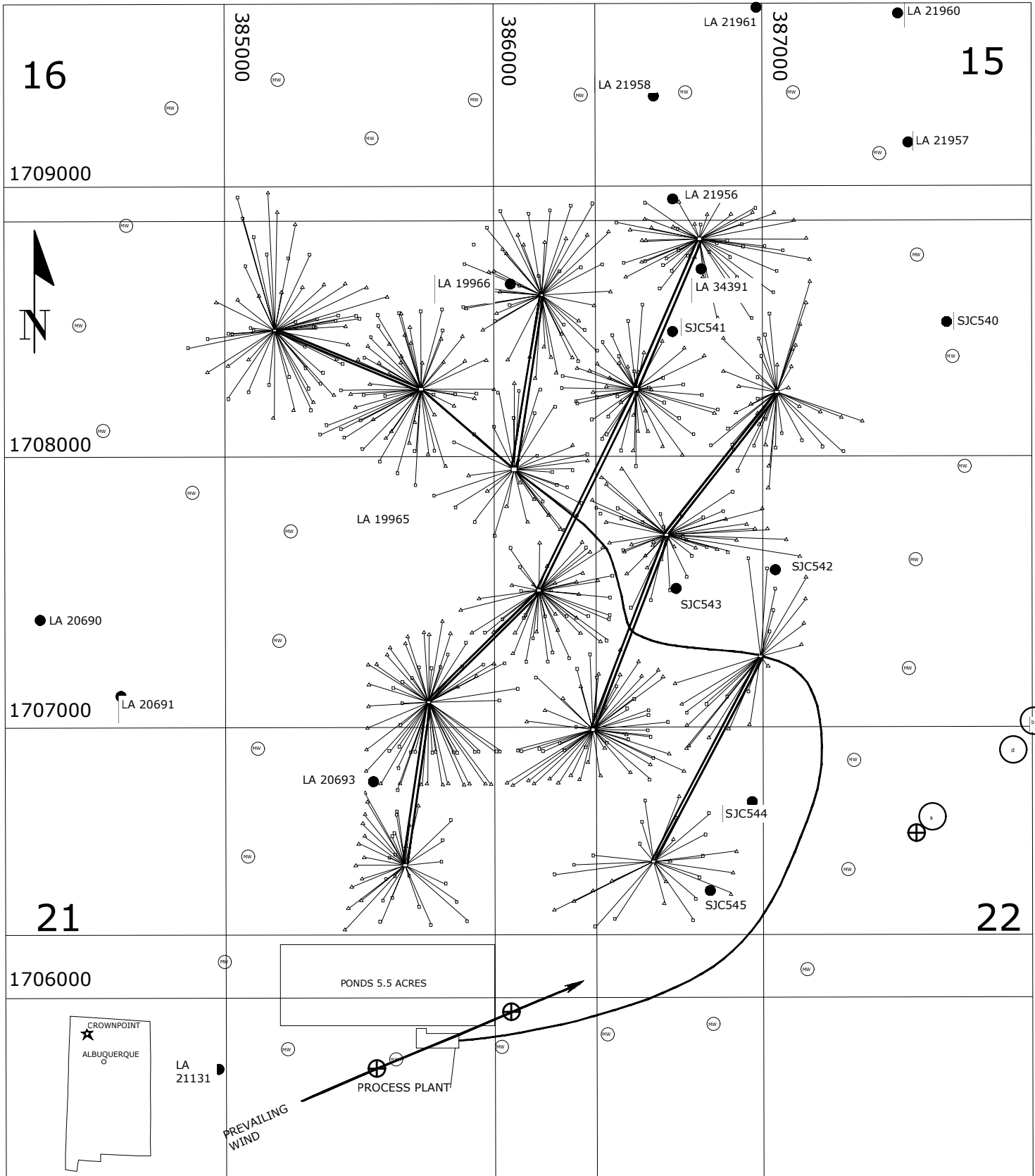
Figure 1.4-8 Proposed Wellfield Site Layout Unit 1 Sections 15, 16, 21 & 22 McKinley County, NM March 1993
