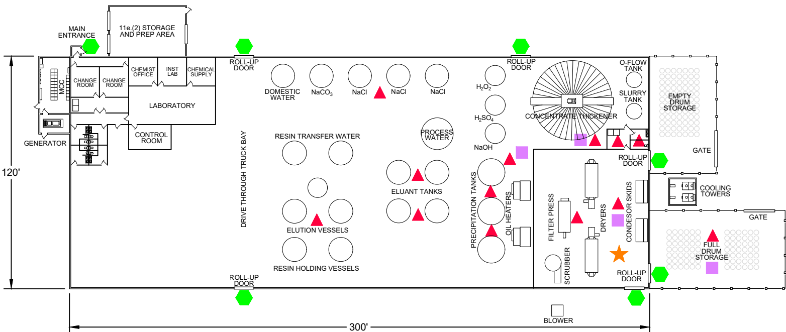
Figure 2.1-1. Schematic of Crownpoint Uranium Process Facility.
