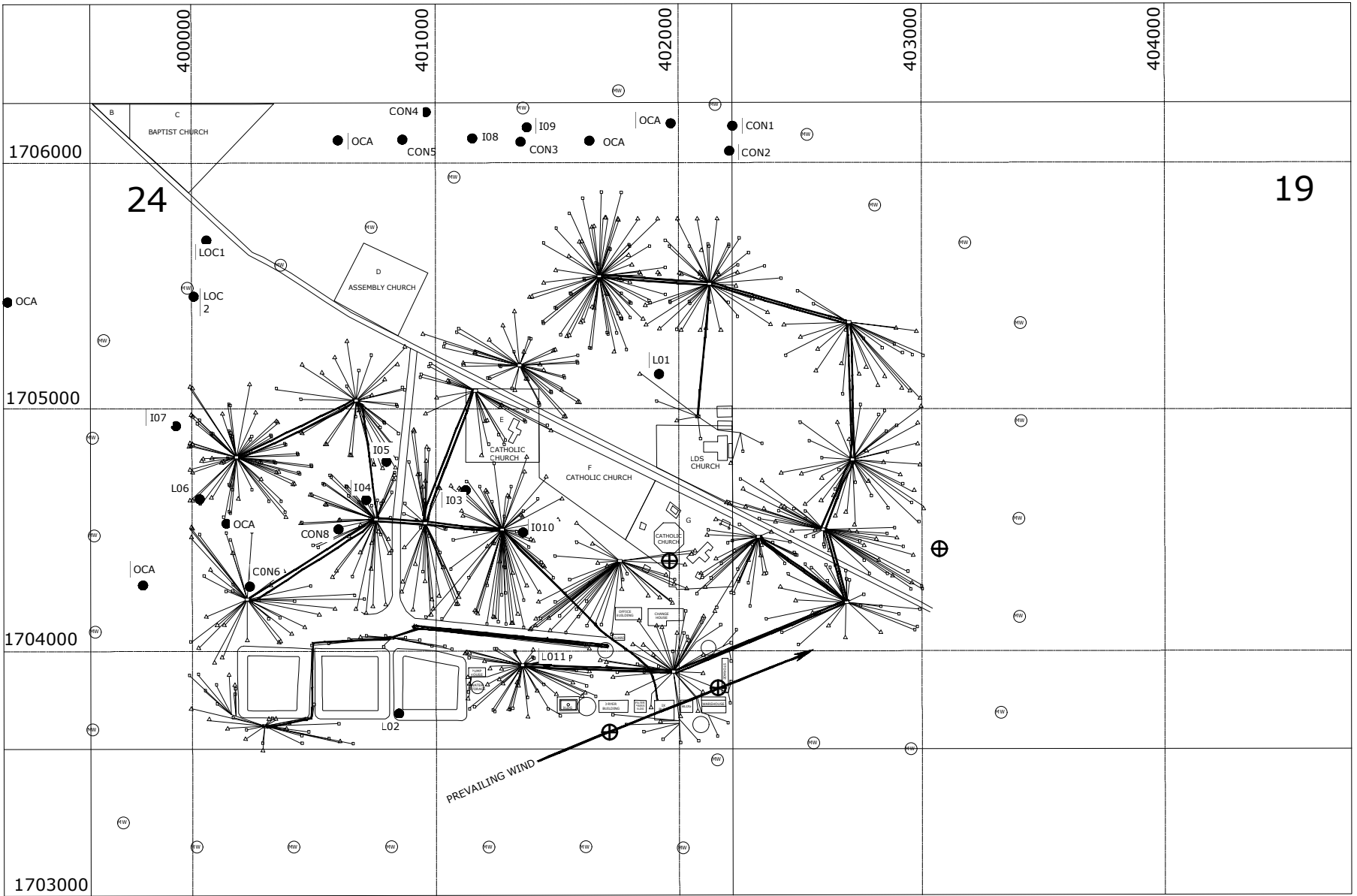
Figure 1.4-6 Proposed Wellfield Site Layout Crownpoint Sections 24 & 19 McKinley County, NM March 1993
