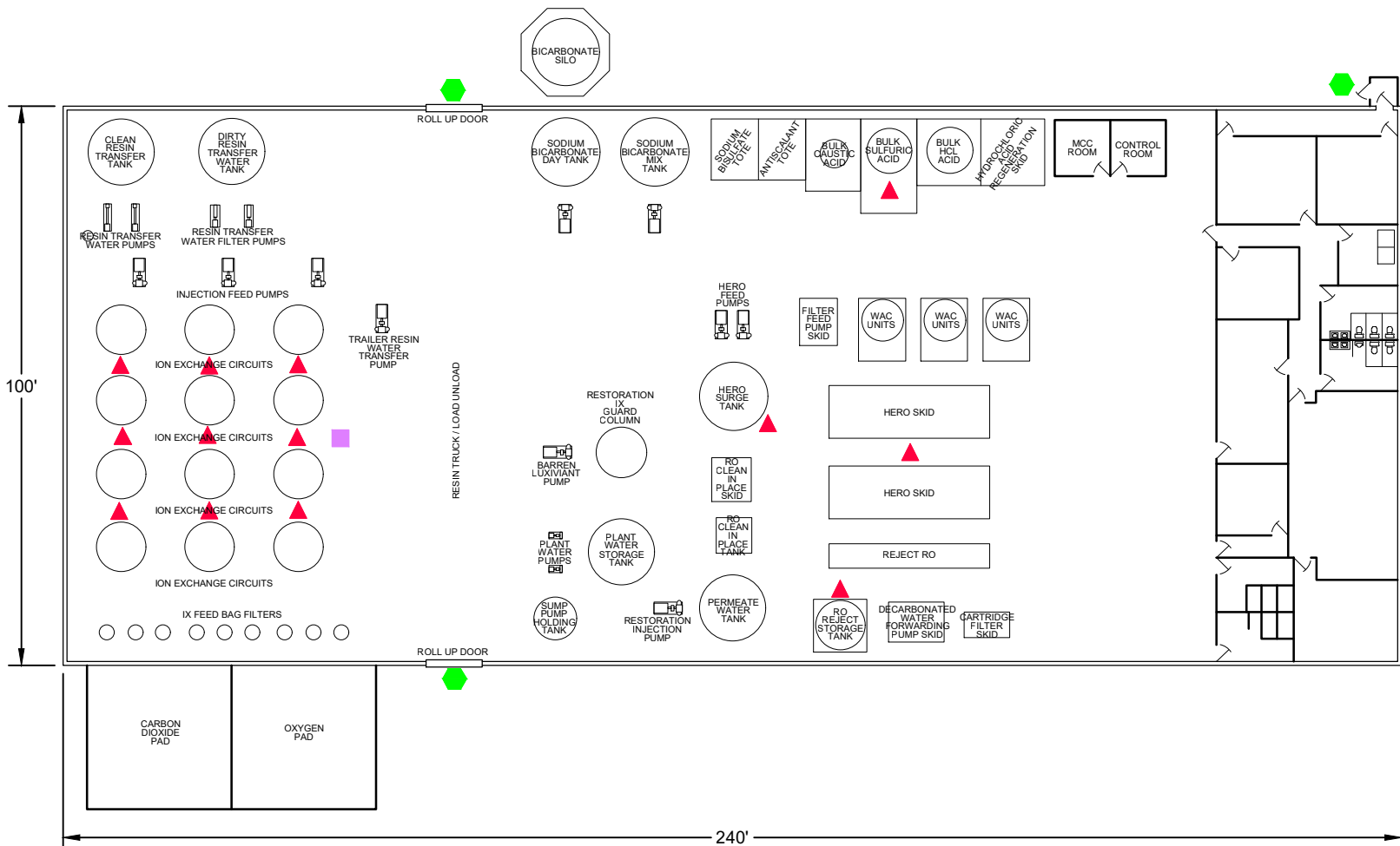
Figure 2.1-2. Schematic Drawing Church Rock Section 8 & Unit 1 Satellites.
