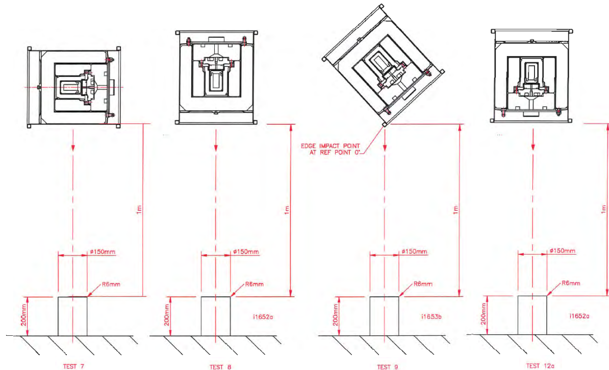
Figure 2-4 Puncture Tests Impact Orientations
