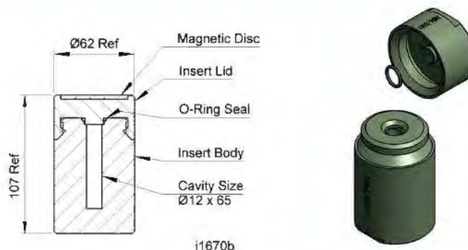
Figure 1-7 Shielding insert LS-12x65-Tu – Design # 3984
