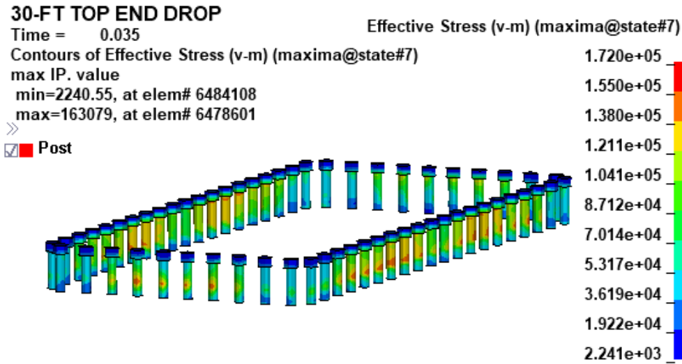
FIGURE 2.7.18 EFFECTIVE STRESS IN THE CLOSURE LID BOLTS – ADDITIONAL HAC TOP END DROP
