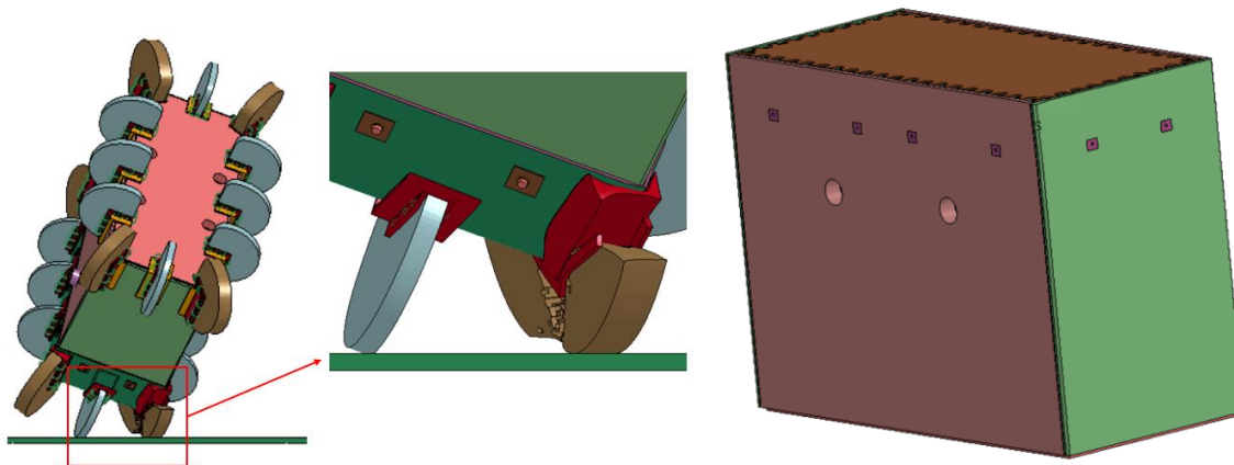
FIGURE 2.7.6 PHYSICAL STATE OF THE CASK SUBSEQUENT TO THE DROP EVENT – TOP CGOC DROP
