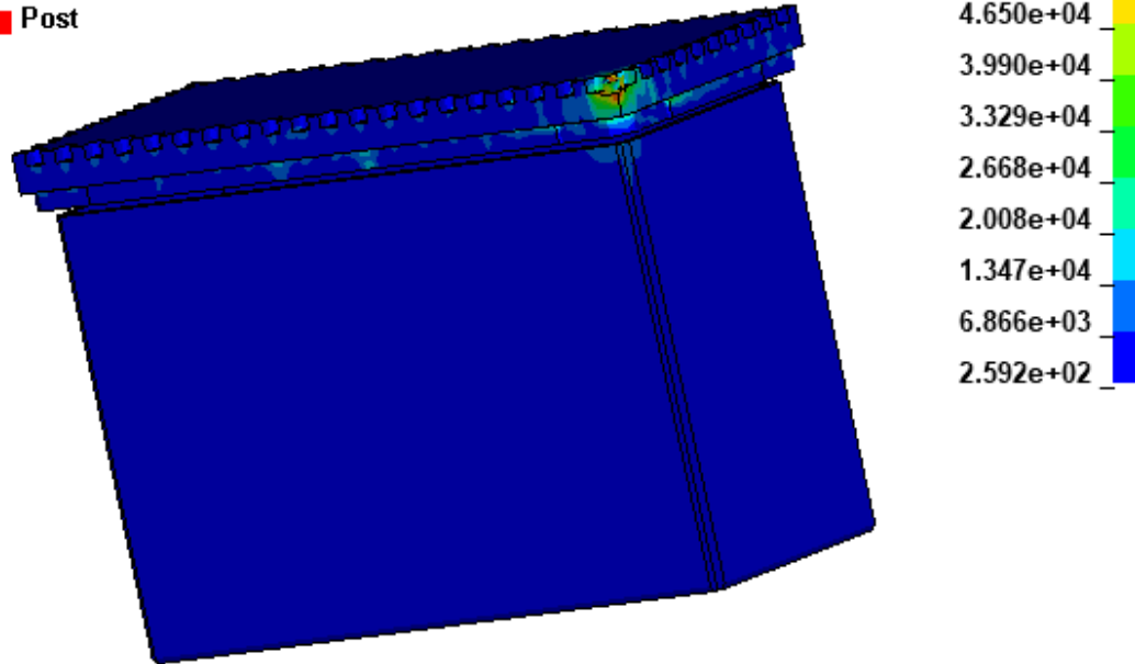
FIGURE 2.7.16 MAXIMUM SHEAR STRESS IN THE CONTAINMENT AT THE END OF INCLINED DROP (TOP END) FOLLOWED BY 1-M PUNCTURE DROP
