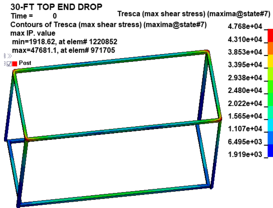
FIGURE 2.7.19 MAXIMUM SHEAR STRESS IN THE CONTAINMENT WELDS – ADDITIONAL HAC TOP END DROP
