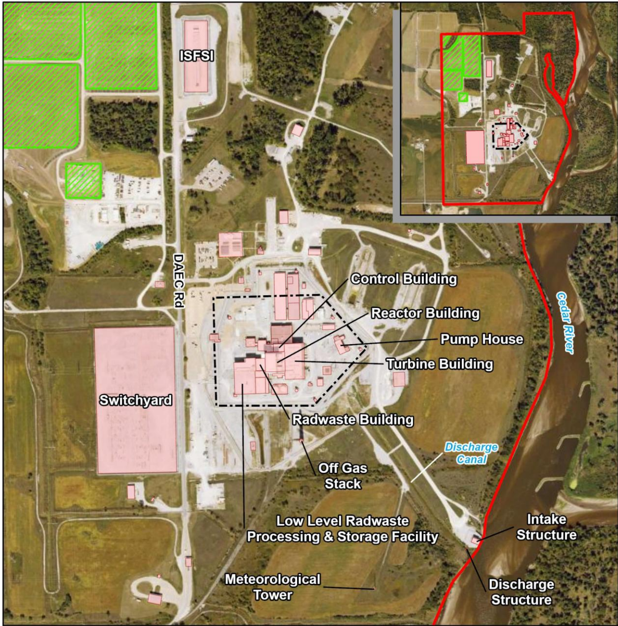
Figure 2 – A map of the Duane Arnold Energy Center site layout from the 2025 Environmental Report (see Figure 2.1-2 in ML25315A003 ).
