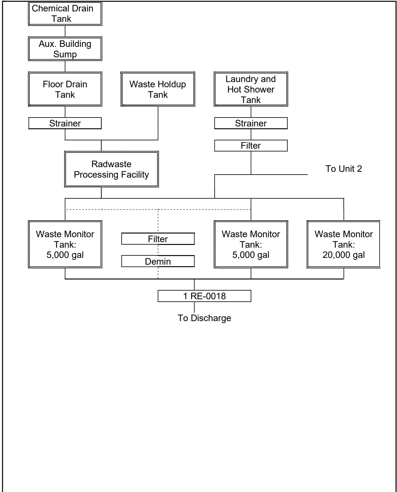
Figure 2-1. Unit 1 Liquid Radwaste Treatment System
