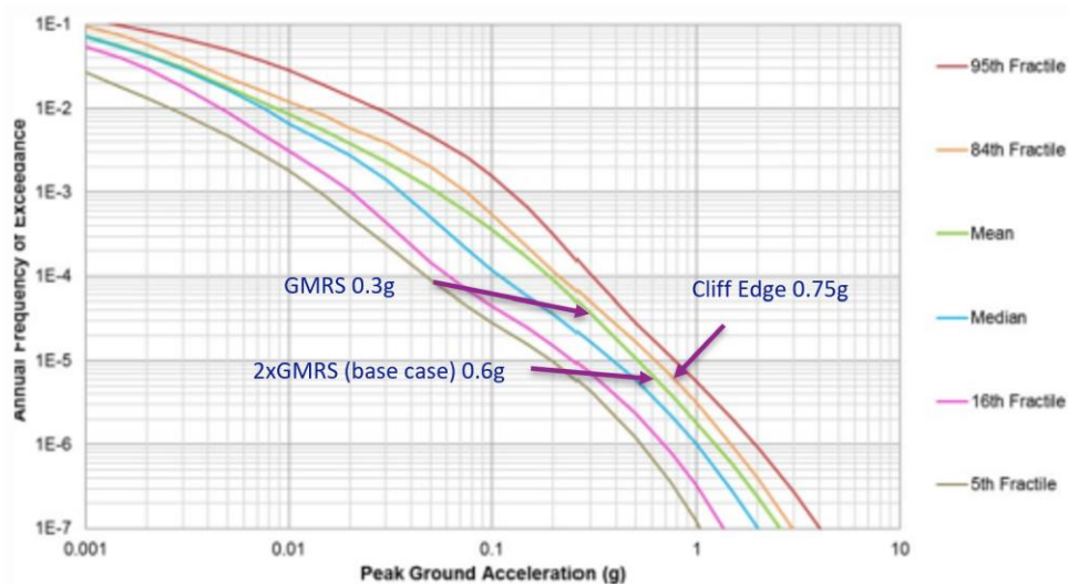
Figure 10.1: Example of Selecting the Cliff Edge Earthquake
