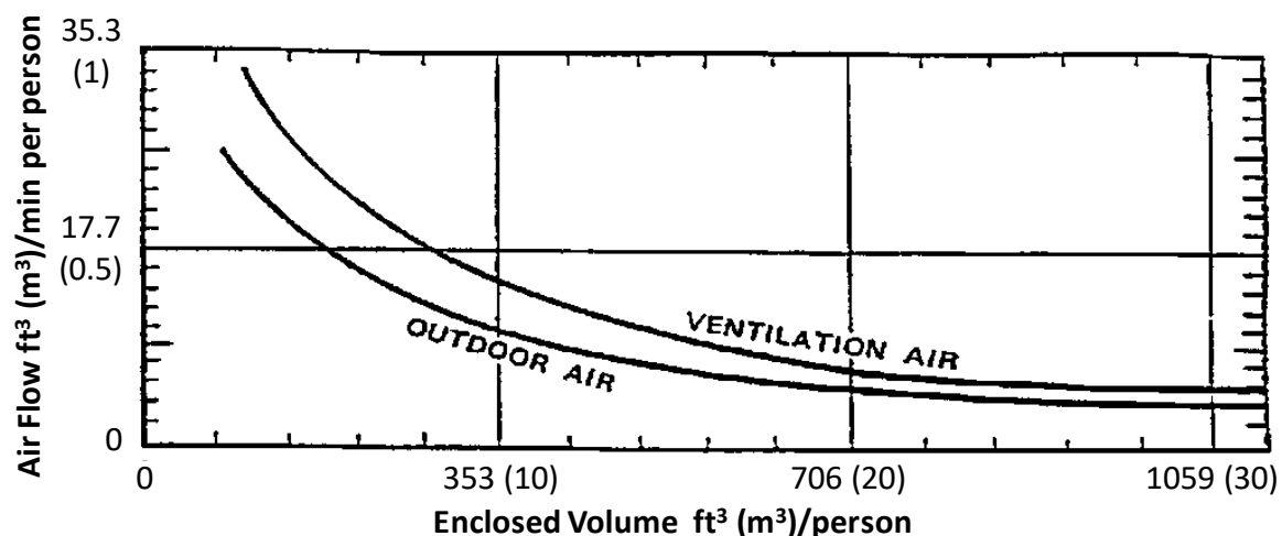
Figure 12.4 Minimum Ventilation Requirements (Source: Figure 34 in MIL-STD 1472G, 2012)
