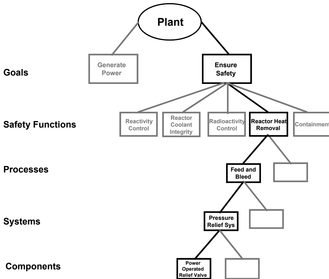
Figure 15.2 Vertical Slice Through an LLWR Plant's Functional Hierarchy for Ensuring Safety
