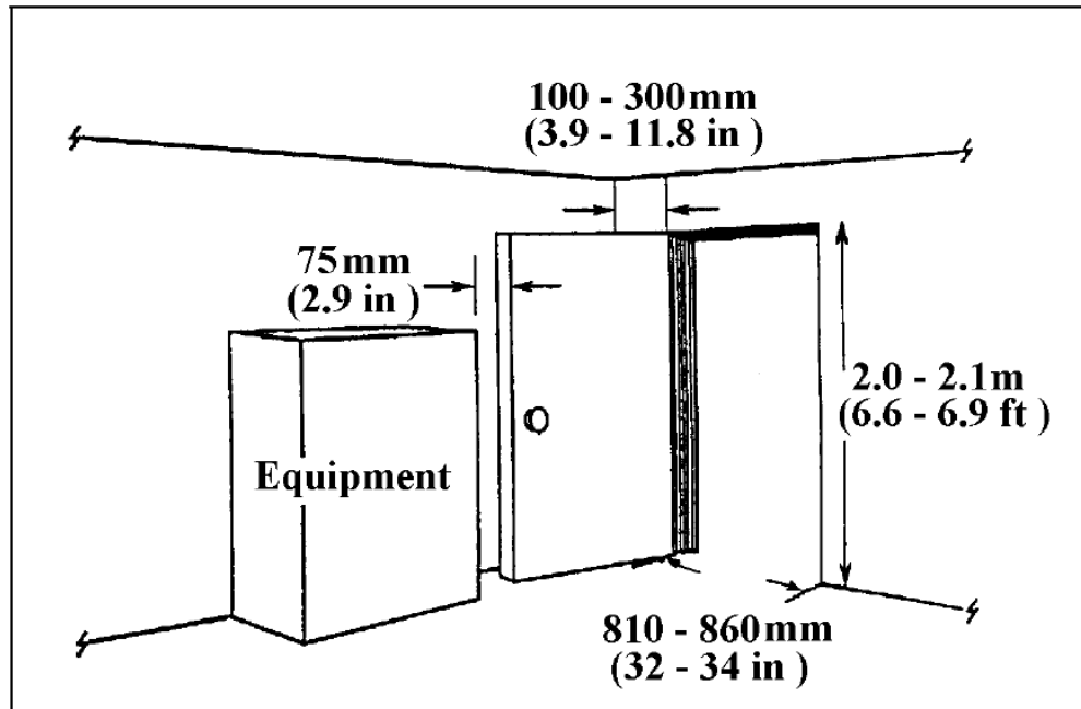
Figure 12.1 Hinged Door Dimensions (Source: Exhibit 10.4.7.2.1 in FAA HFDS, 2003)
