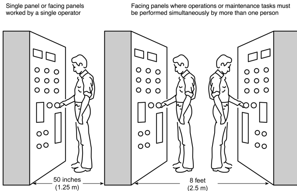
Figure 12.3 Equipment-To-Equipment Distances: Single Person And More-Than-One-Person Spaces
