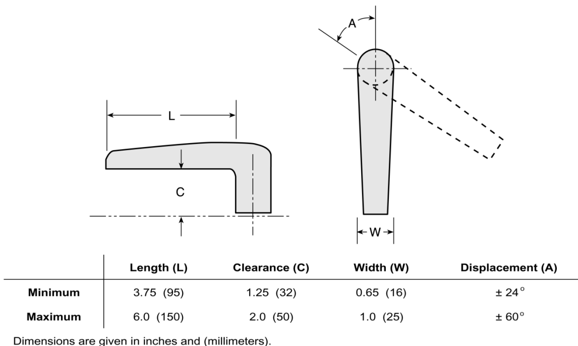
Figure 3.9 High-Torque J-Handle Dimensions
