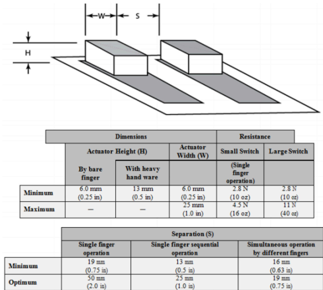
Figure 3.5 Recommended Dimensions for Slide Switches
