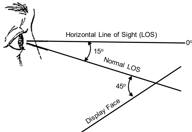
Figure 11.2 Line Of Sight (Source: Figure 2 in MIL-STD-1472G, 2012)
