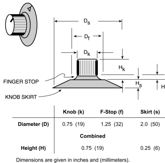
Figure 3.11 Recommended Dimensions for Rotary Controls with Finger Stops and Skirts
