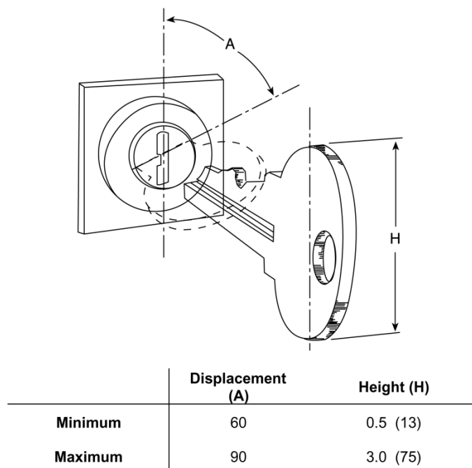
Figure 3.10 Key-Operated Control Dimensions
