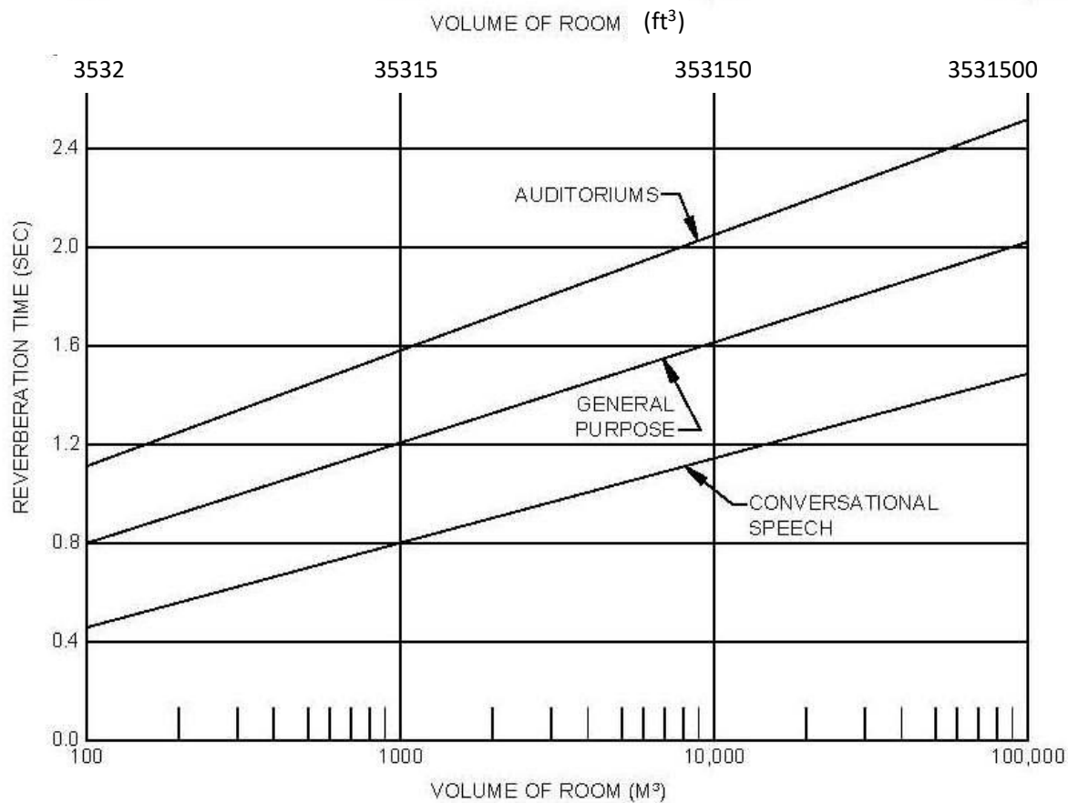
Figure 12.6 Acceptable Reverberation Times (Source: Figure 39 in Mil-Std-1472G, 2012)
