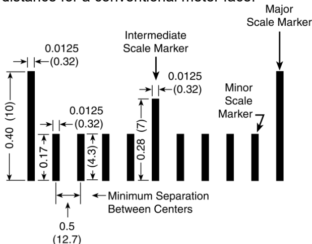
Figure 1.10 Graduation Dimensions in Inches (Millimeters) for a 3-Foot (0.9 Meter) Viewing Distance
