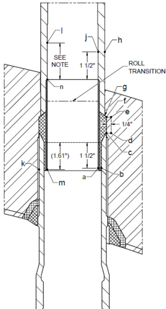
Figure 4-3 Nozzle Examination (CRDM nozzle 8)
