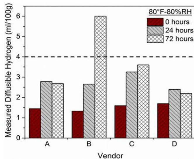
Figure 2. Graph showing slight increase of diffusible hydrogen after exposure of 24 and 72 hours [6]
