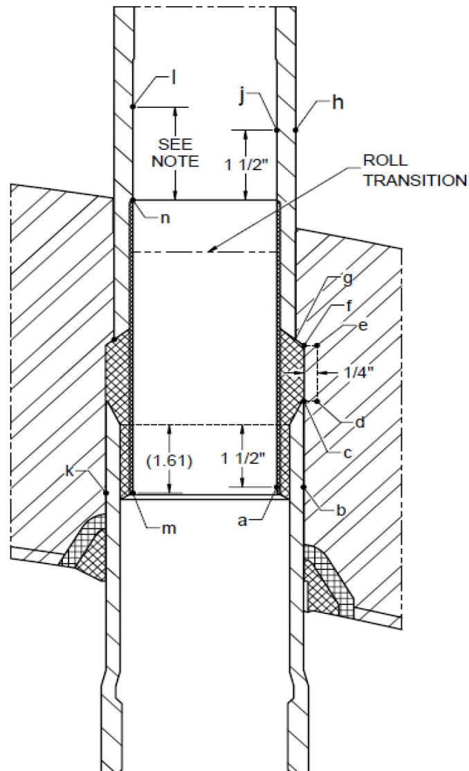
Figure 3-3 Nozzle Examination (CRDM Nozzle 4)
