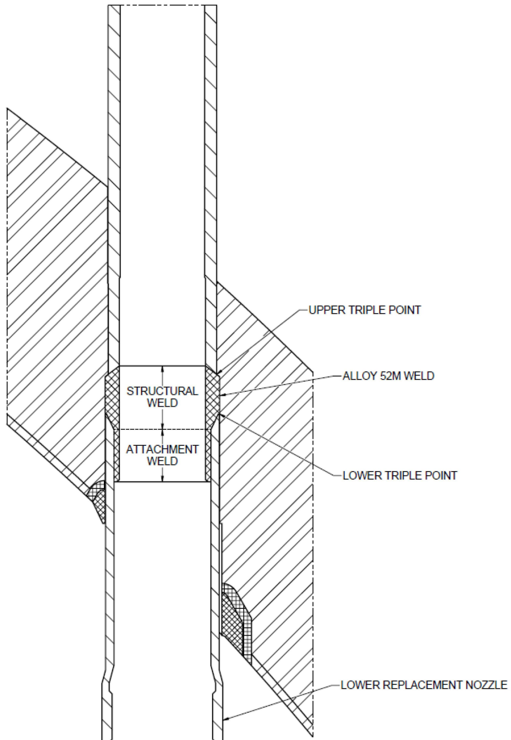
Figure 2 Nozzle Weld
