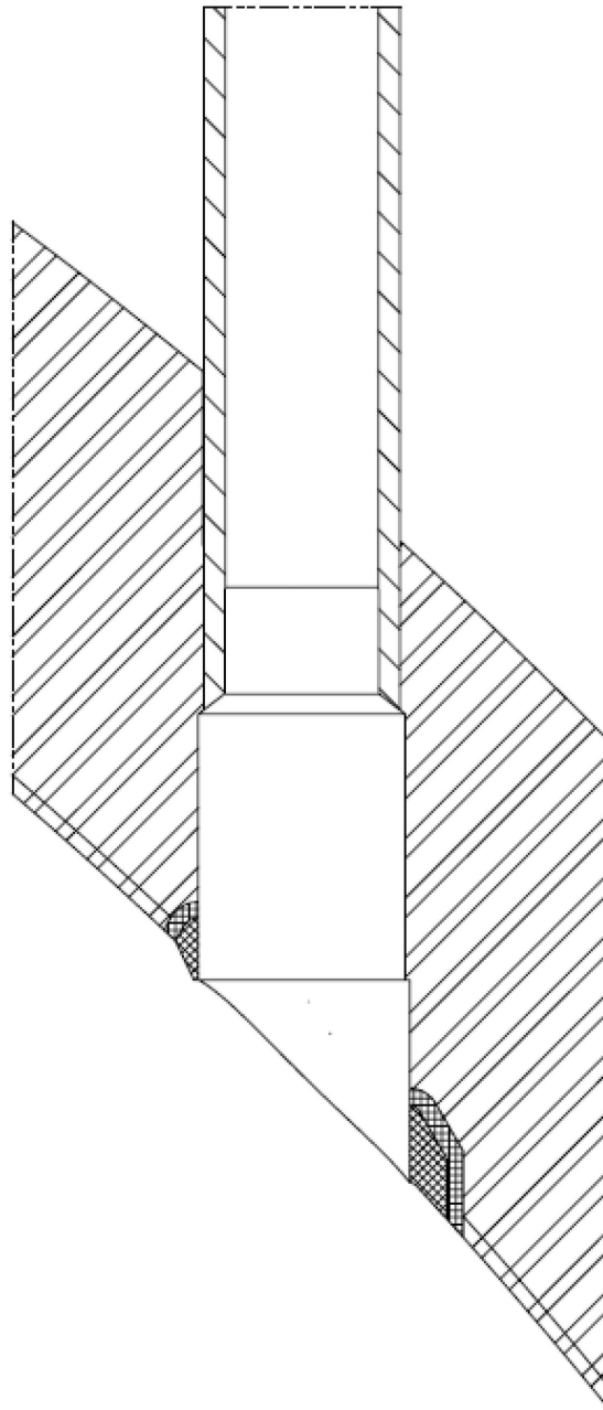
Figure 1 Nozzle Machining
