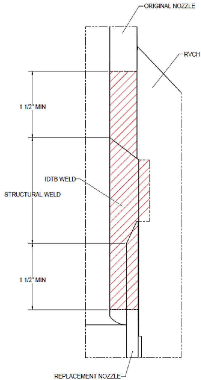
Figure 6 Nozzle 45°L UT Beam Coverage Looking Up
