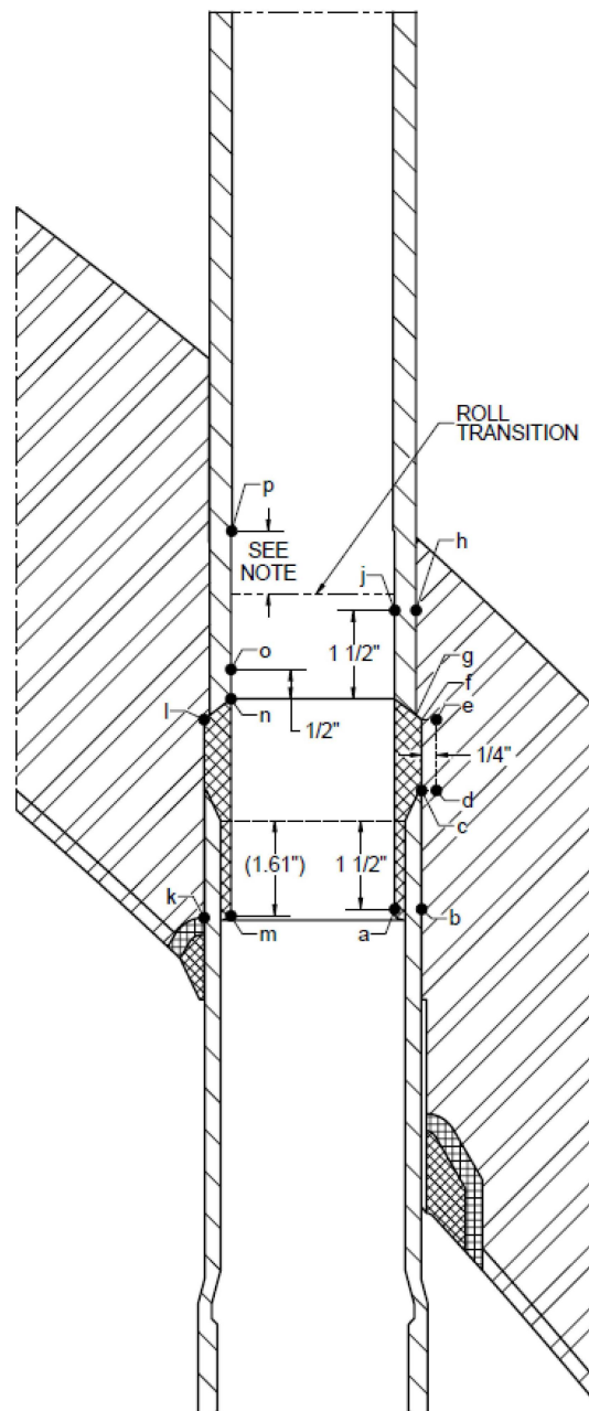
Figure 3 Nozzle / Weld Examination
