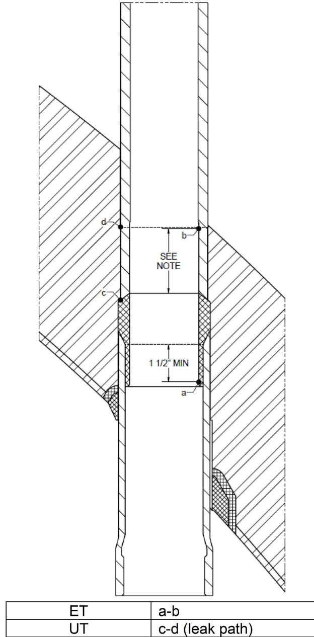
Figure 9 Nozzle PSI / ISI Examination (Applicable for All CRDM / ICI Nozzles Except Those Identified In Figure 10, Nozzle 5, Nozzle 4, and Nozzle 8)
