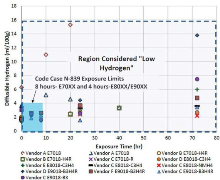
Figure 1. Results of EPRI diffusible hydrogen testing at 27°C 80% Relative Humidity (HR) for zero to 72 hours of exposure [6]
