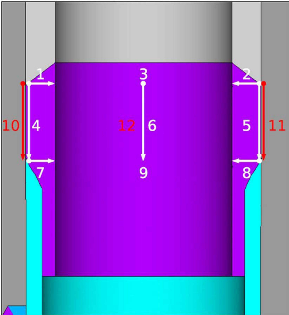
Figure 12 Crack Propagation Paths
