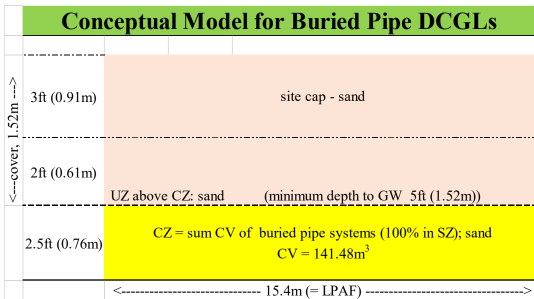
Figure 1: Conceptual Configuration of CV for Embedded Pipes (note: not to scale)
