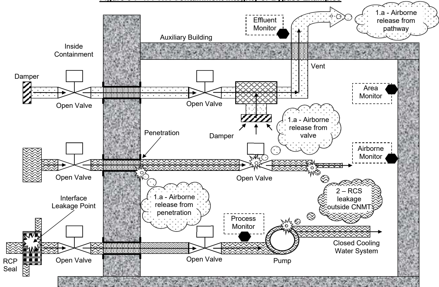
Figure 3-F-1: PWR Containment Integrity or Bypass Examples
