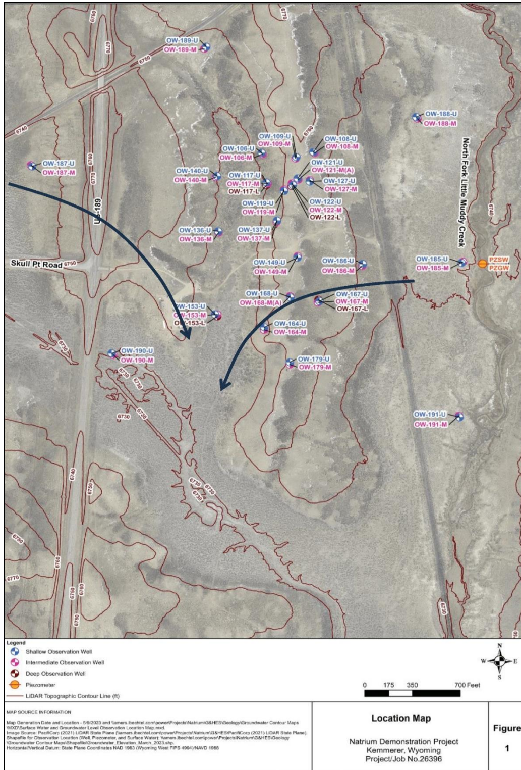
Figure 3-8 Observation Wells Installed at the Kemmerer Unit 1 Site and Generalized Groundwater Flow Paths. Adapted from: TerraPower 2024-TN10896.
