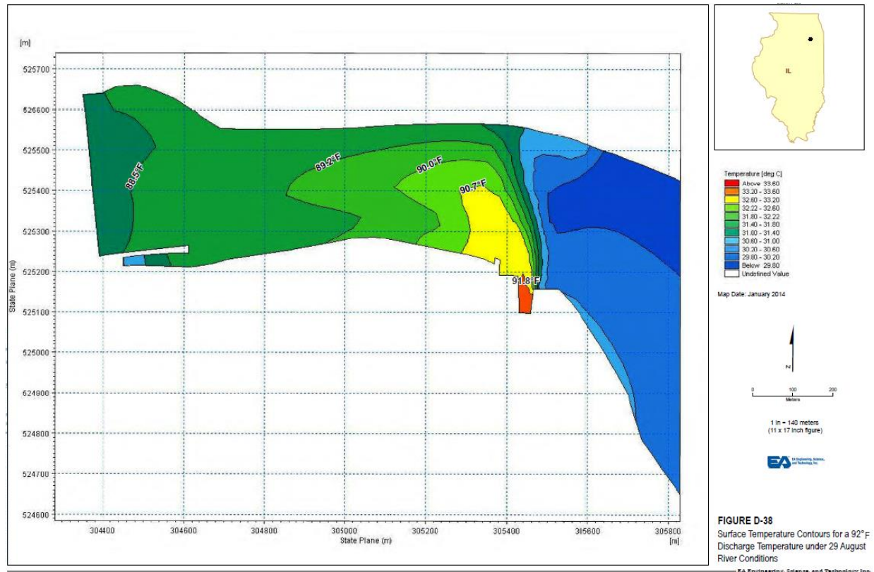
Figure E-2 Surface Temperature Contours for a 92°F Discharge Temperature under August 29, 2013 River Conditions in Dresden Pool. Source: IPCB 2016-TN11816.
