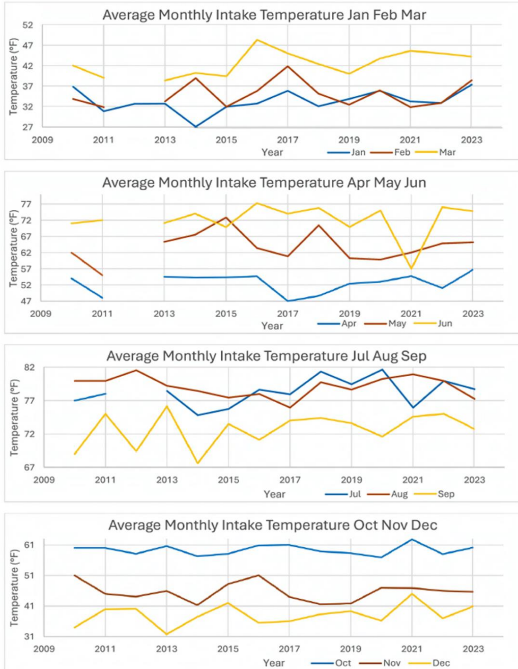
Figure 3-4 Average Monthly Intake Temperature over the 2010 to 2023 Period. Source: CEG 2025-TN11342.
