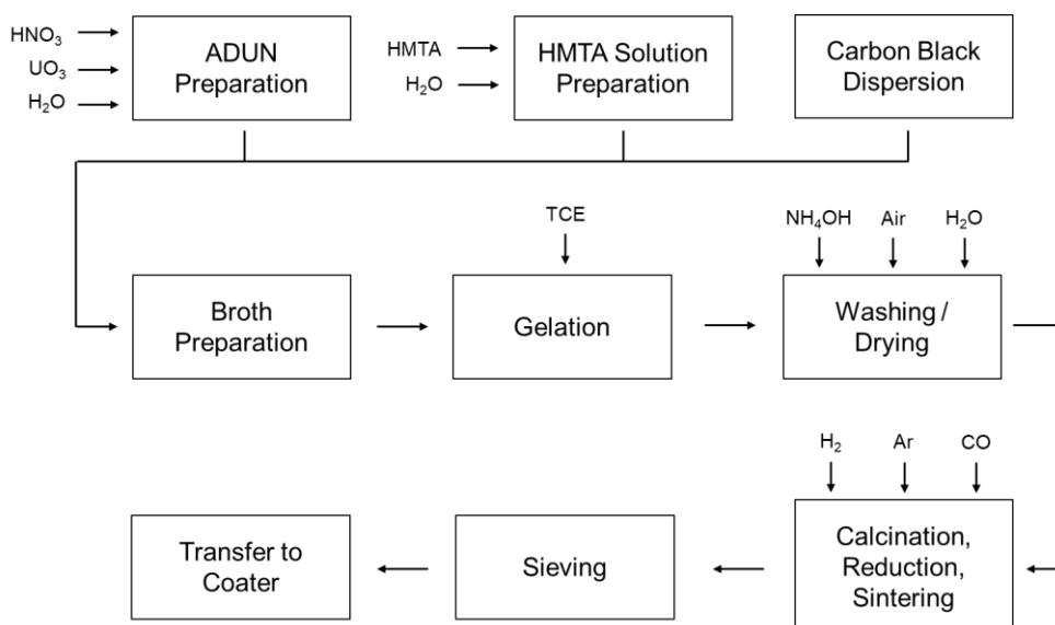
Figure 2. Process Flowsheet for Fabrication of TRISO Fuel Kernels by Internal Gelation per the AGR Fuel Program.
