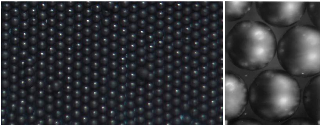
Figure A-4. Sintered UO 2 Kernels of 500–532 μm Diameter (Collins et al. 2004).
