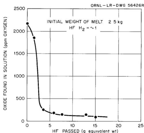
Figure B-1. Measured Oxide Content in \text{LiF}\text{-}\text{BeF}_2 (63–37 mol.%) Following Treatment with \text{HF}\text{-}\text{H}_2 Mixtures at 700^\circ\text{C} (Shaffer 1971).
