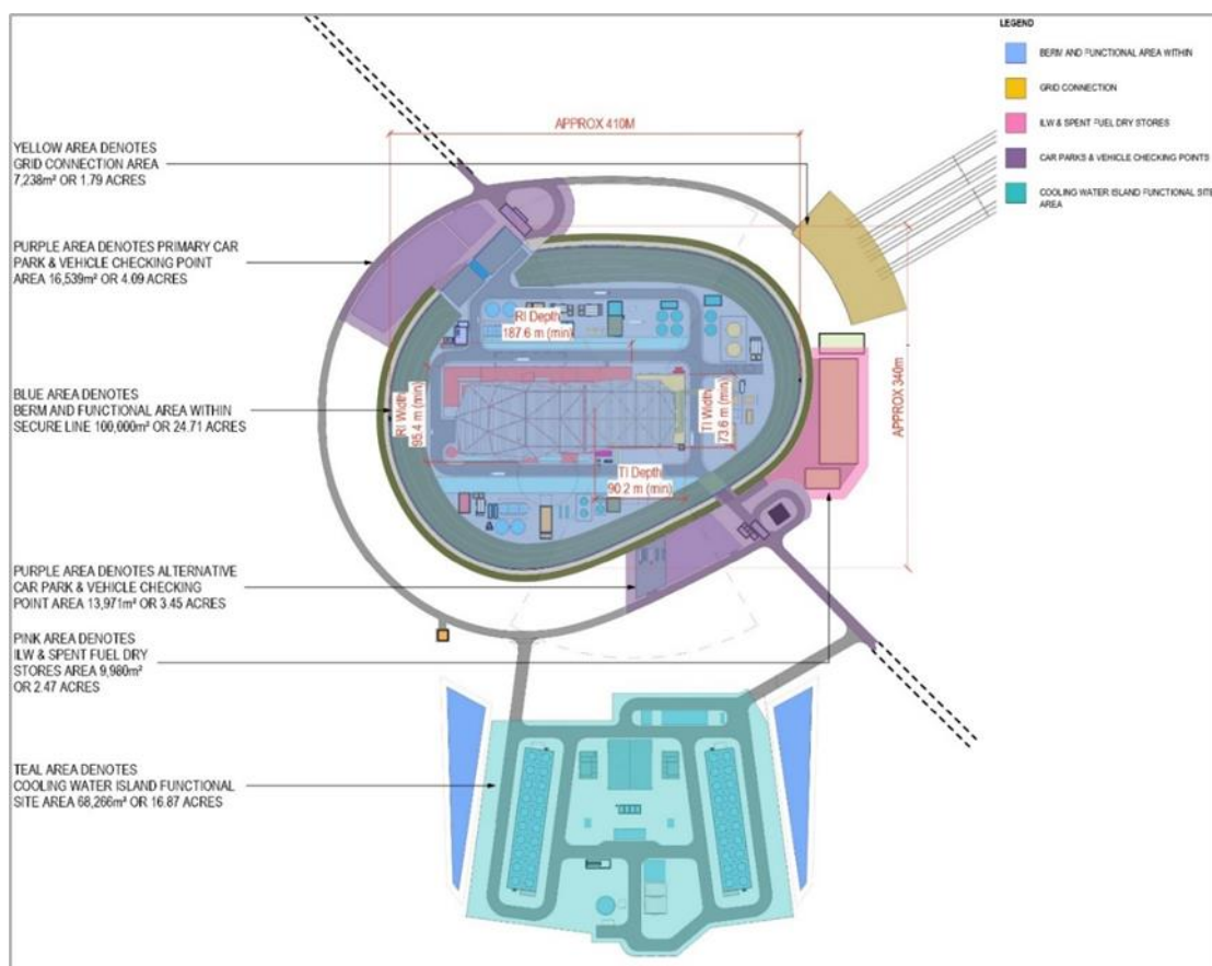
Figure 6 – Site Layout
