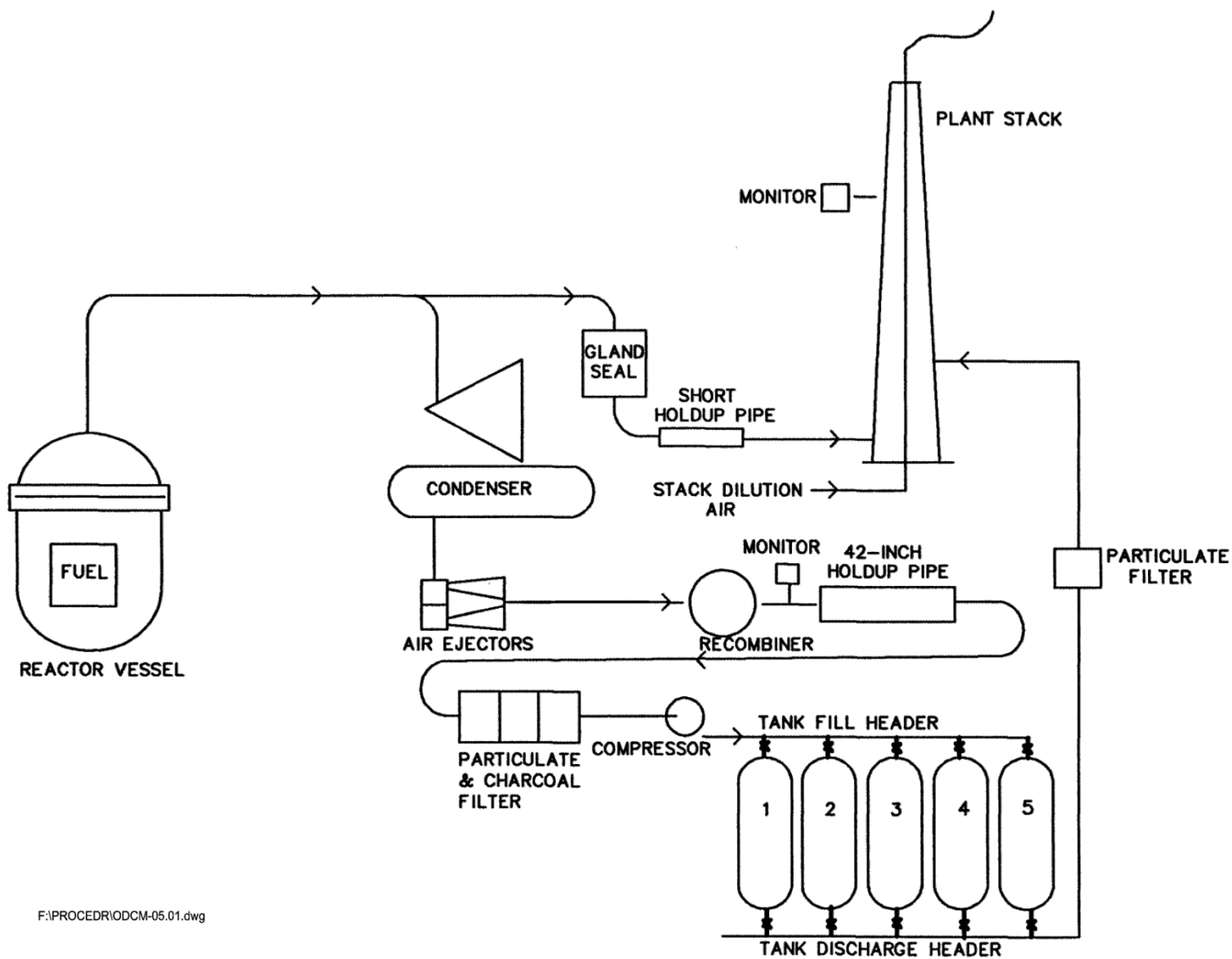
Figure 1 Gaseous Radwaste
