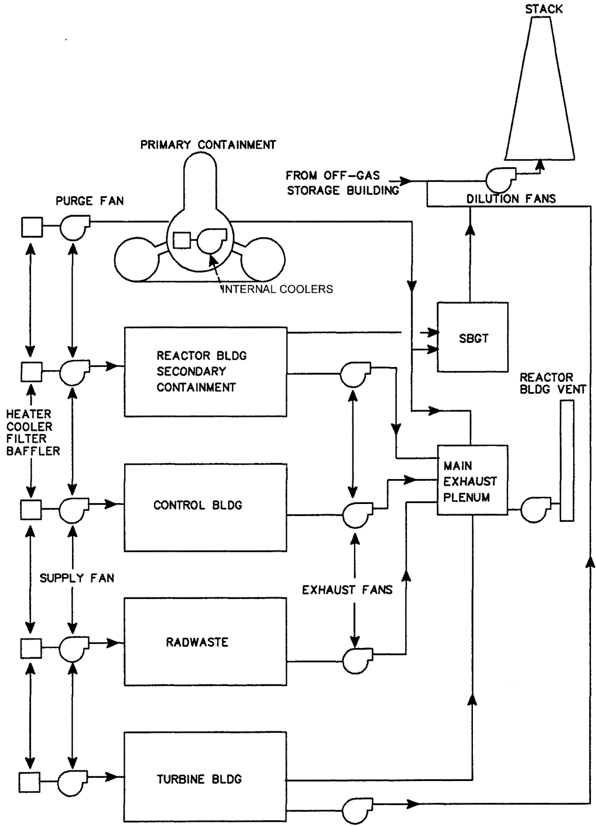
Figure 2 Ventilation System
