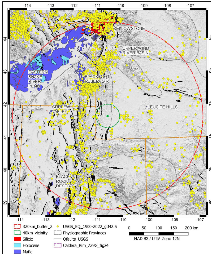
Figure 1: Reproduced from TR Figure 14 showing the location of the proposed site relative to faults, regional seismicity, and Quaternary volcanic rocks in the site region 4
