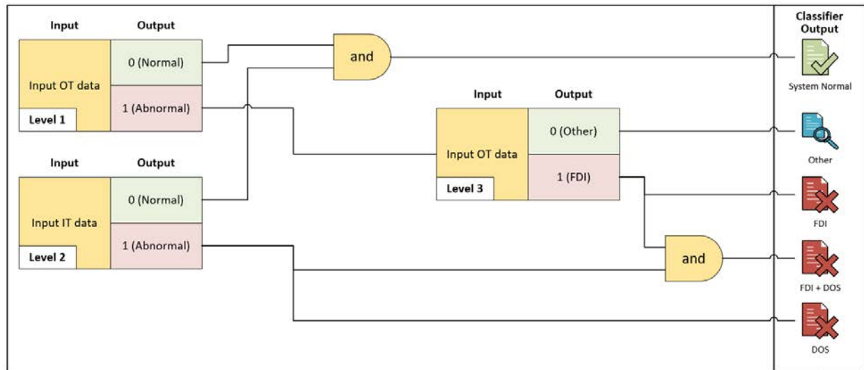
Figure 13. Implemented composite classifier.
