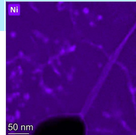
As-printed, 376 °C irradiation to 2 dpa
