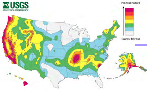
Pre-binned seismic hazard (6 zones, 2 soils)
