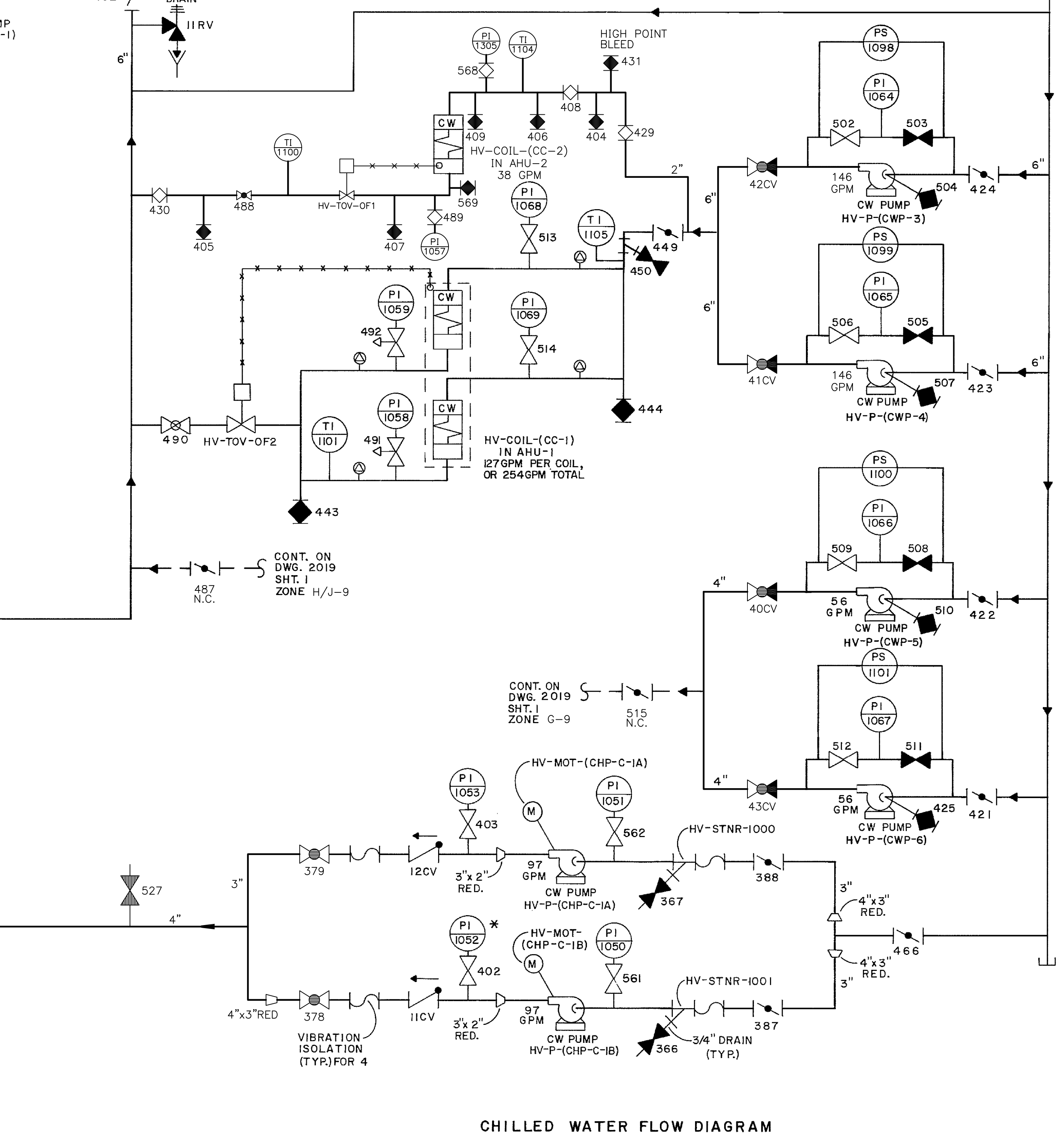
CHILLED WATER FLOW DIAGRAM
