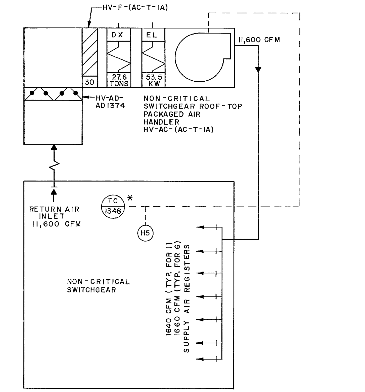
NON-CRITICAL SWITCHGEAR ROOF-TOP HVAC
