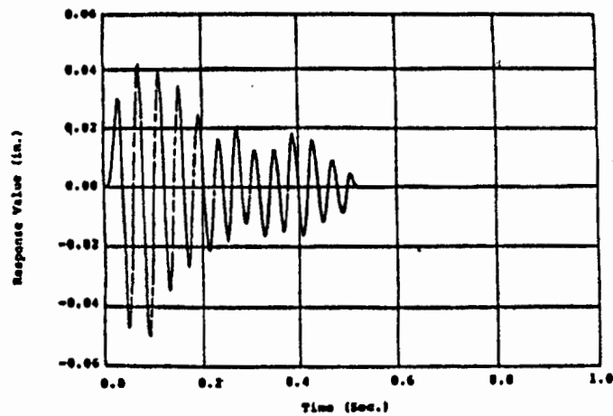
RESPONSE 2 FOR CDF 2 HIGH PRESSURE CORE INJECTION LINE Y DISPLACEMENT DUE TO CHUGGING
