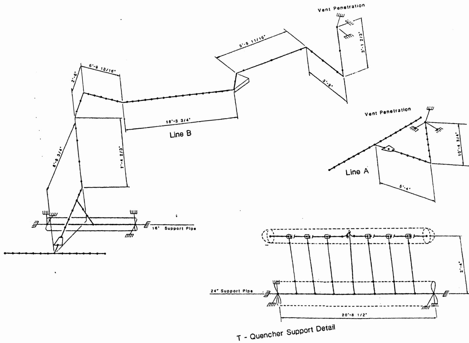
FIGURE 5.2 S/RVD LINE MODELS (WETWELL ROUTING)
