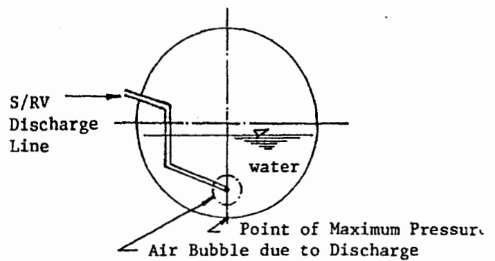
Section View of the Torus
