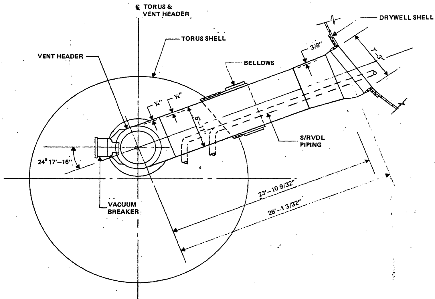
SECTION - VENT SYSTEM
