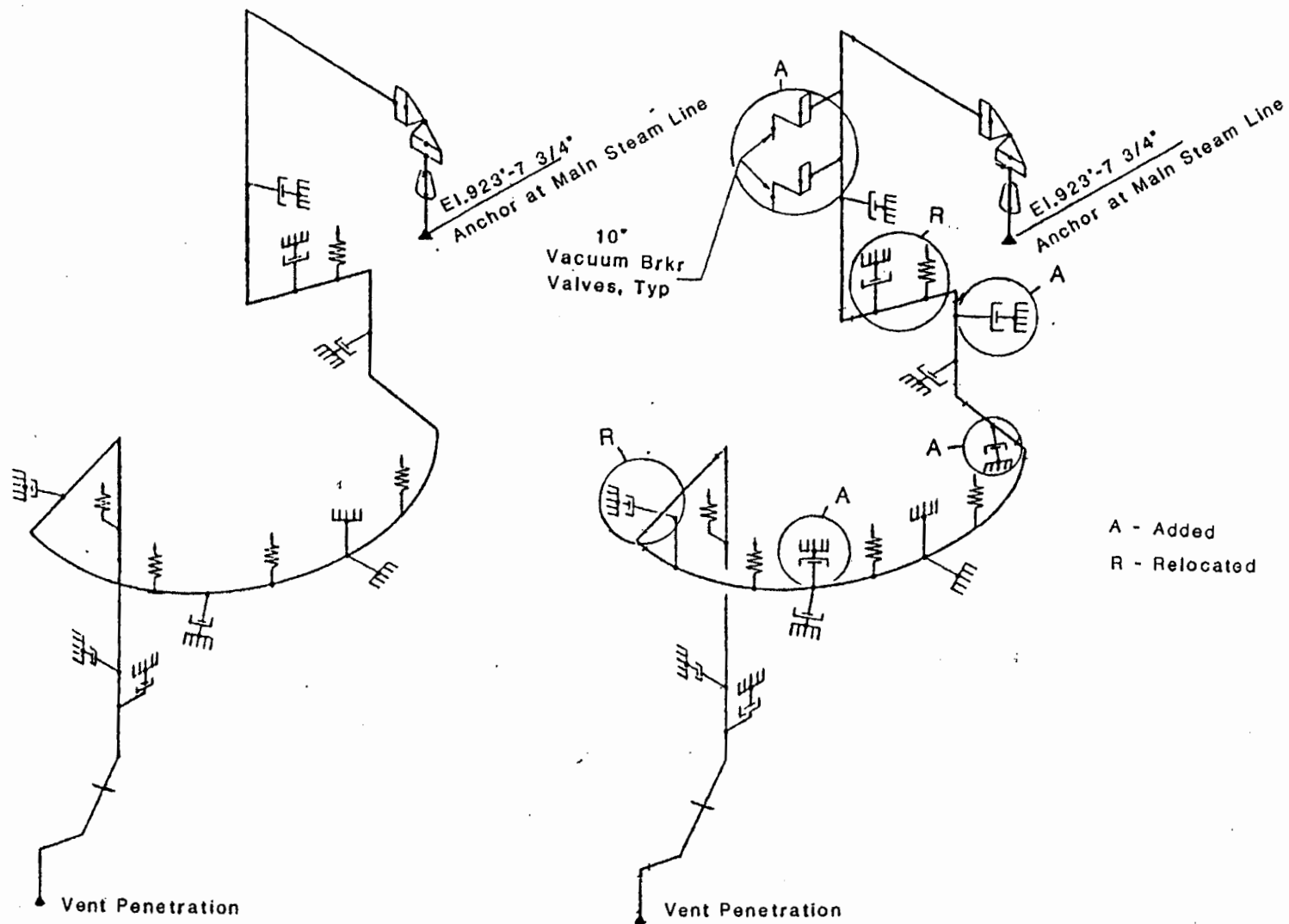
FIGURE 5.1 REPRESENTATIVE DRYWELL S/RVD LINE MODEL (LINE 71G) BEFORE AND AFTER MODIFICATIONS
