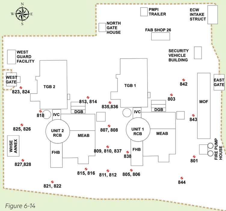
STP Protected Area Ground Water Monitoring Wells
