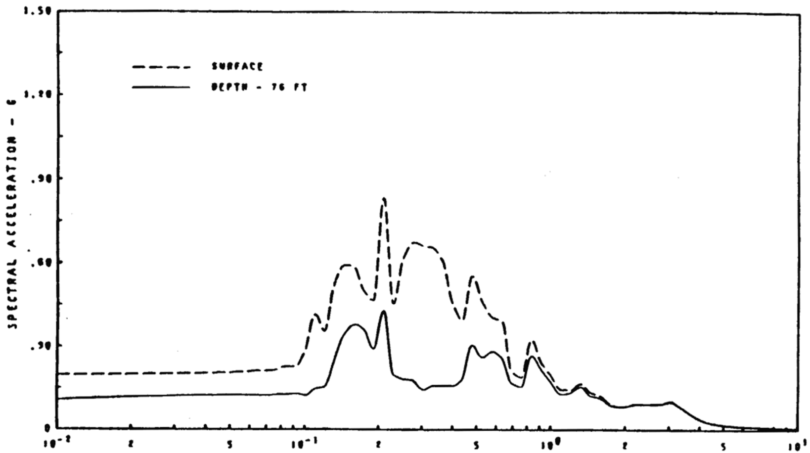
RESPONSE SPECTRA - 2. PER. DAMPING OLYMPIA HWY LAB N06E 1949
