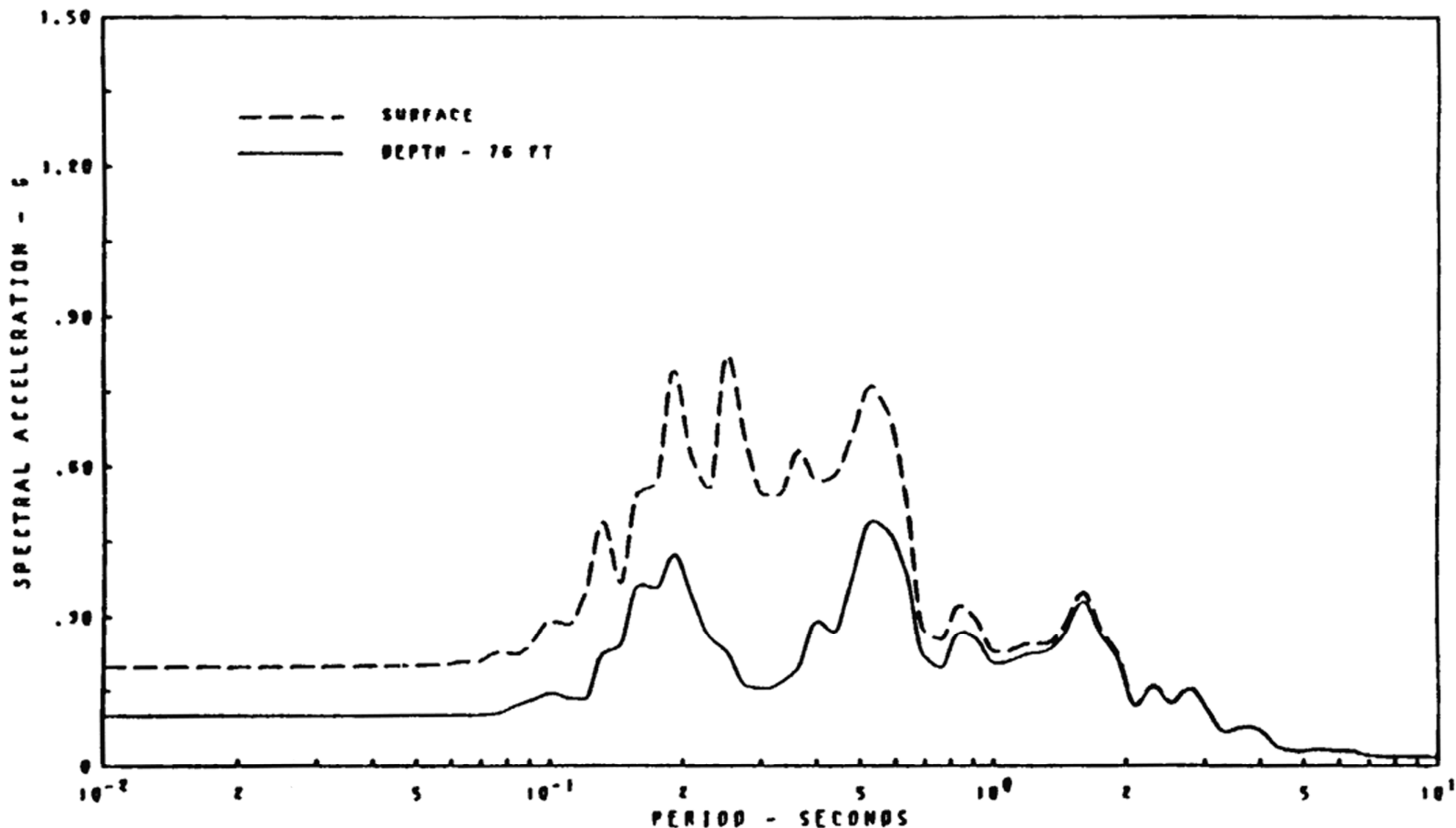
RESPONSE SPECTRA - 2. PER. DAMPING SAN LUIS OBISPO 564W PARKFIELD 1966 REV 14 10/07
