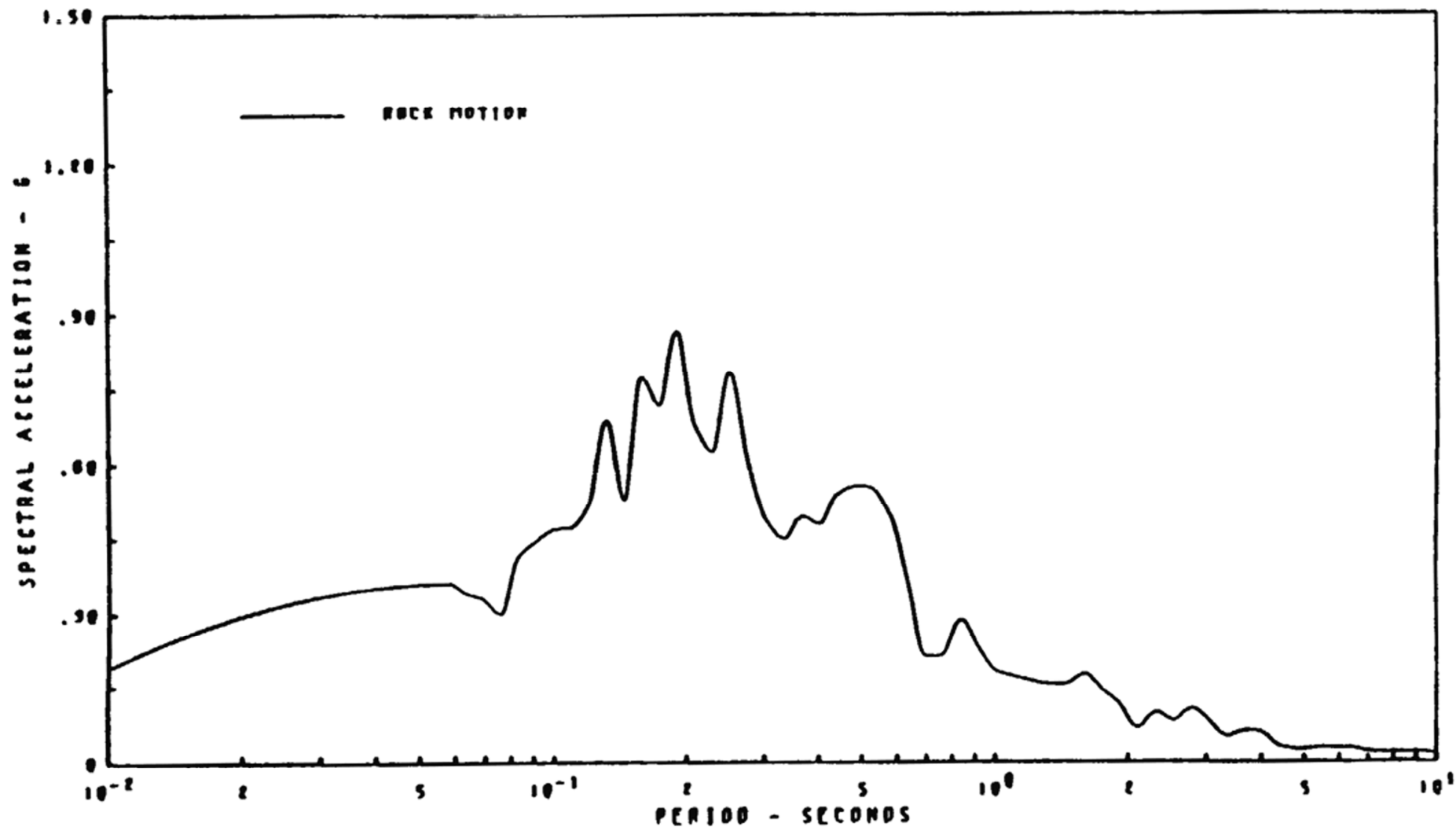
RESPONSE SPECTRA - 2. PER. DAMPING SAN LUIS OBISPO 564W PARKFIELD 1966
