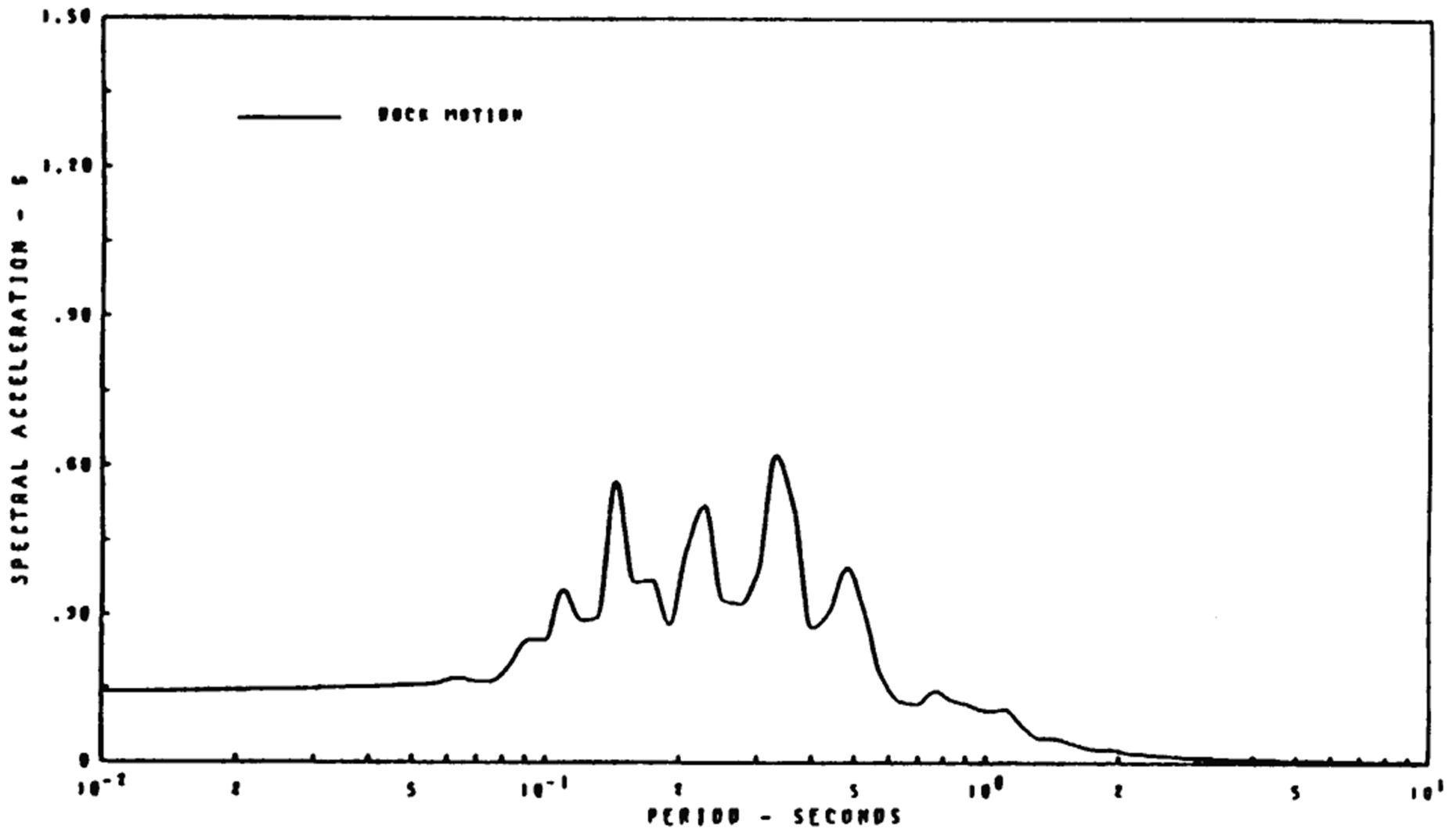
RESPONSE SPECTRA - 2. PER. DAMPING CASTAIC S. FERNANDO 1971
