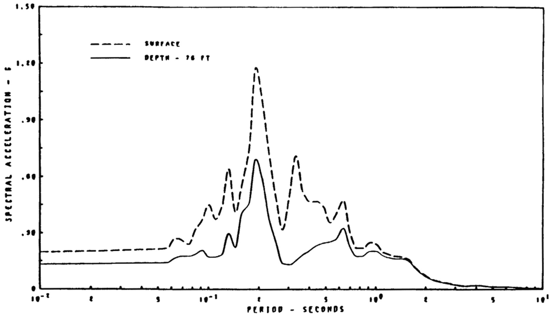
RESPONSE SPECTRA - 2. PER. DAMPING LAKE MICH. NO. 4 S. FERNANDO 1971
