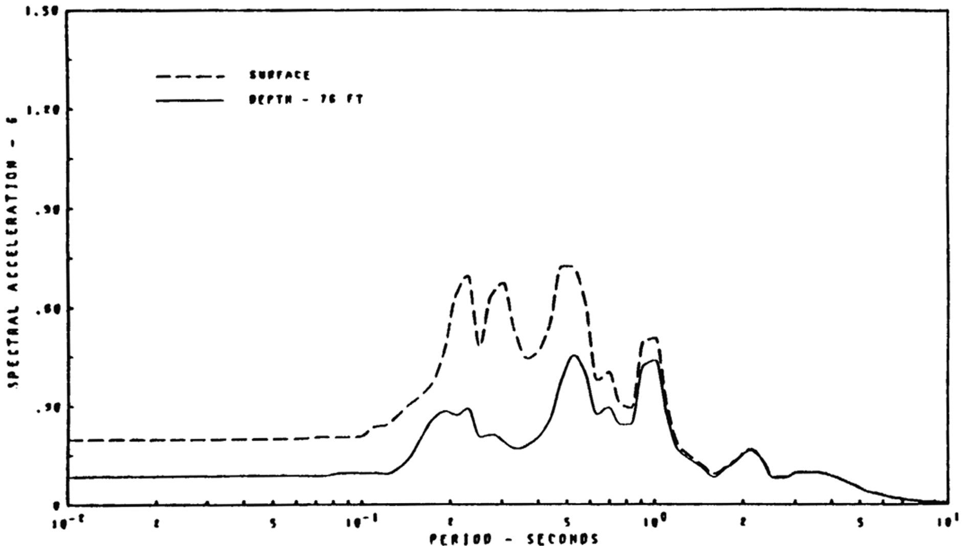
RESPONSE SPECTRA - 2. PER. DAMPING GRAFFITH PARK SOW S. FERNANDO 1971
