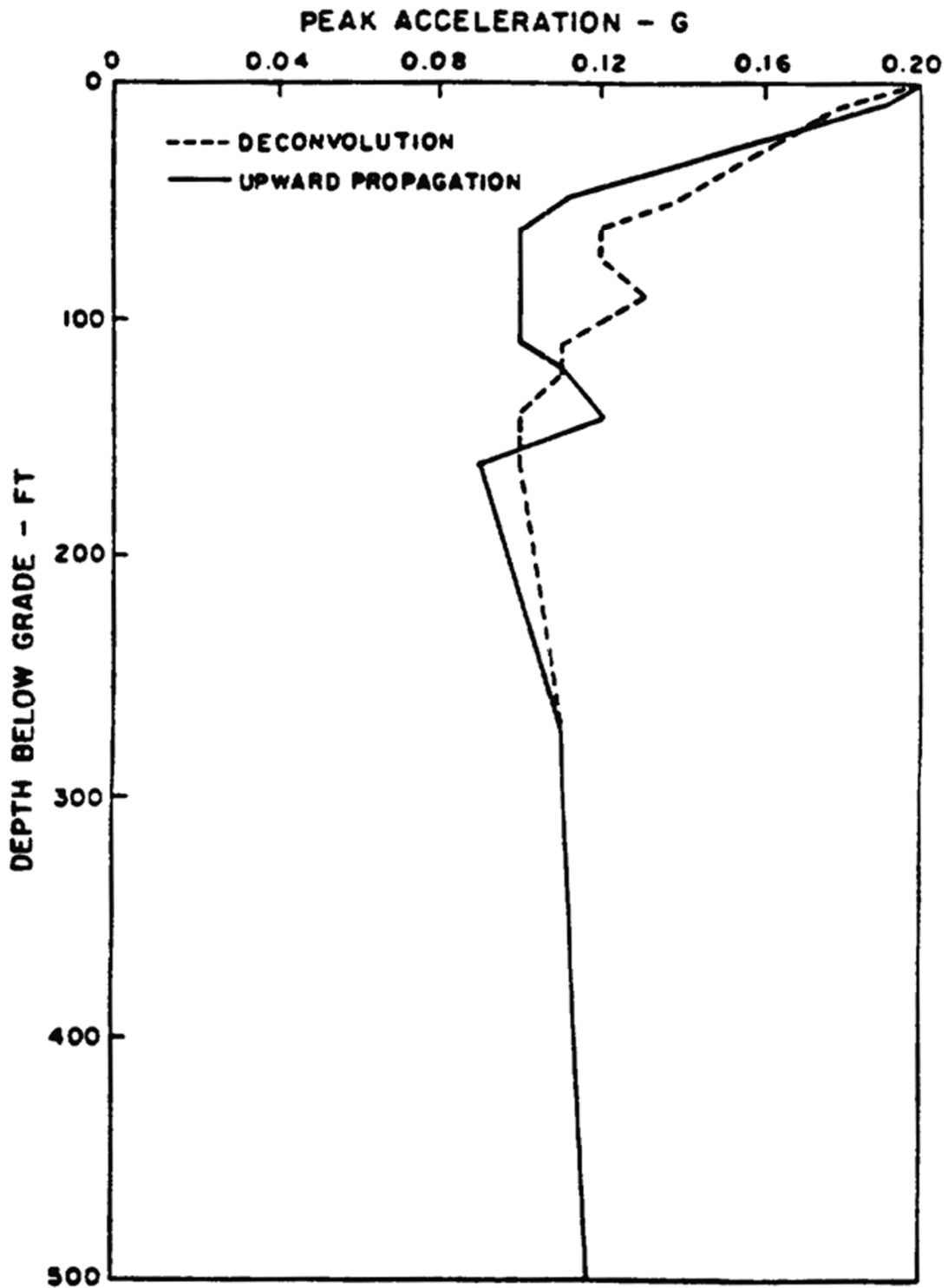
VARIATION OF MEAN PEAK ACCELERATION WITH DEPTH OF DECONVOLUTION AND UPWARD PROPAGATION ANALYSES
