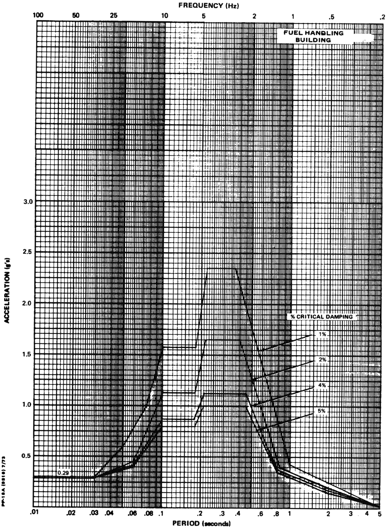
OPERATING BASIS EARTHQUAKE VERTICAL ACCEL. RESPONSE SPECTRA EL. 220 FT 0 IN. FIGURE 3D-58
