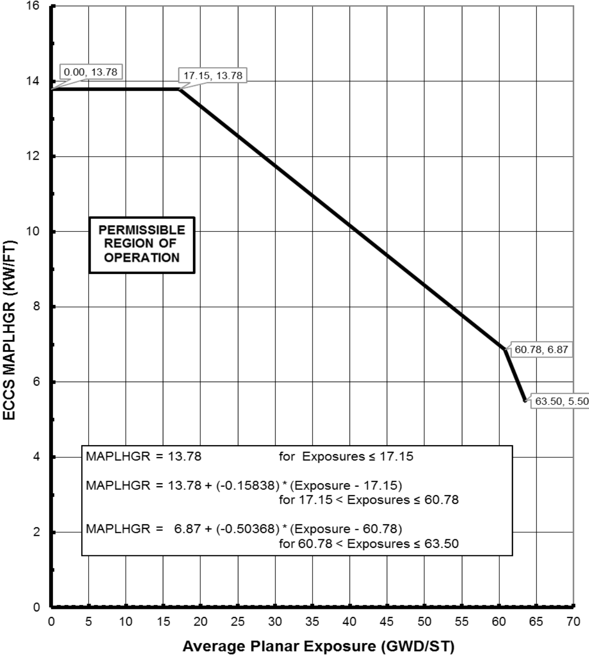
Figure 3.2.1-1 MAPLHGR Versus Average Planar Exposure
