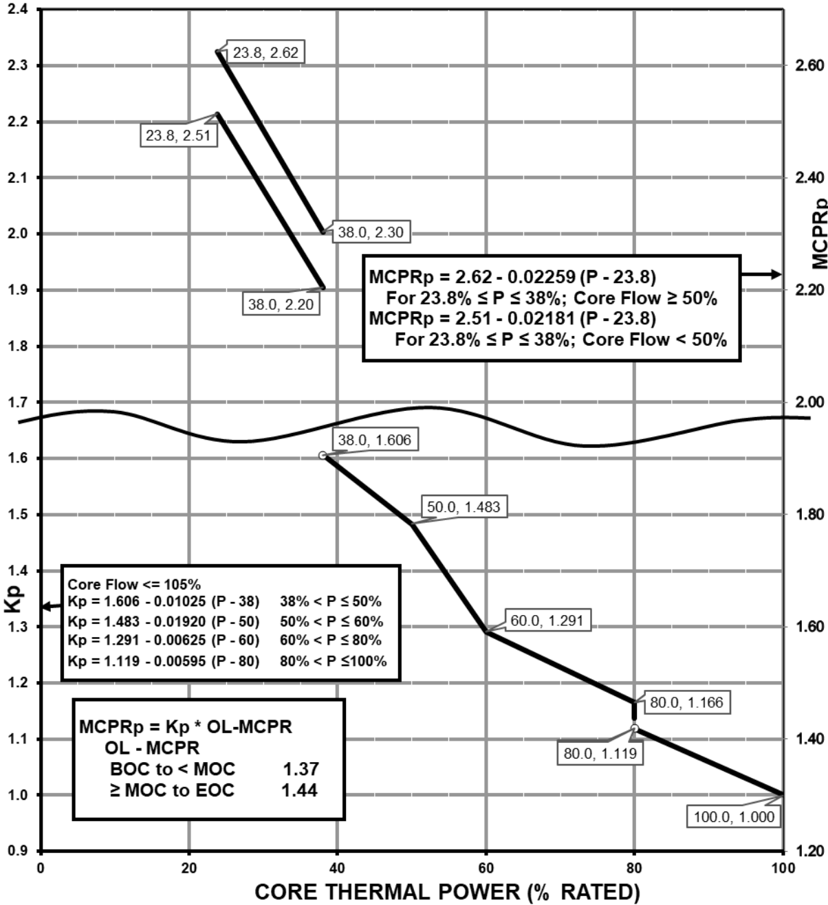
Figure 3.2.2-3 Power Dependent MCPR Limit (MCPR p ) Pressure Regulator Out of Service
