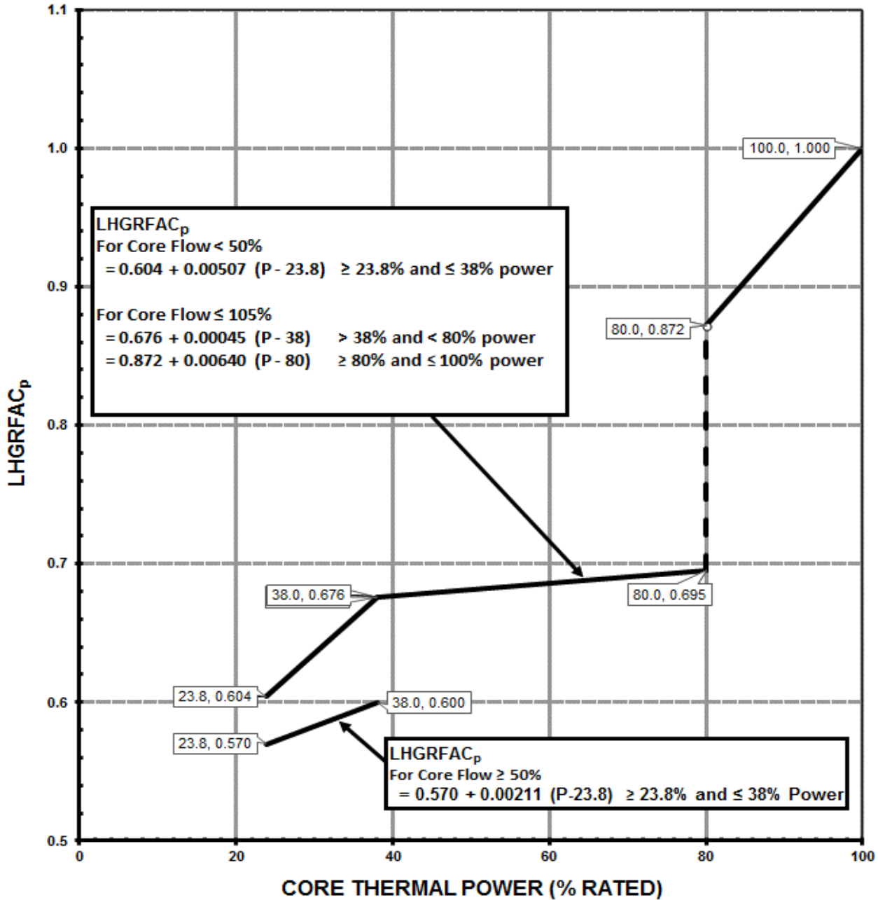
Figure 3.2.3-3 Power Dependent LHGR Factor (LHGRFAC p ) Power Load Unbalance Out of Service
