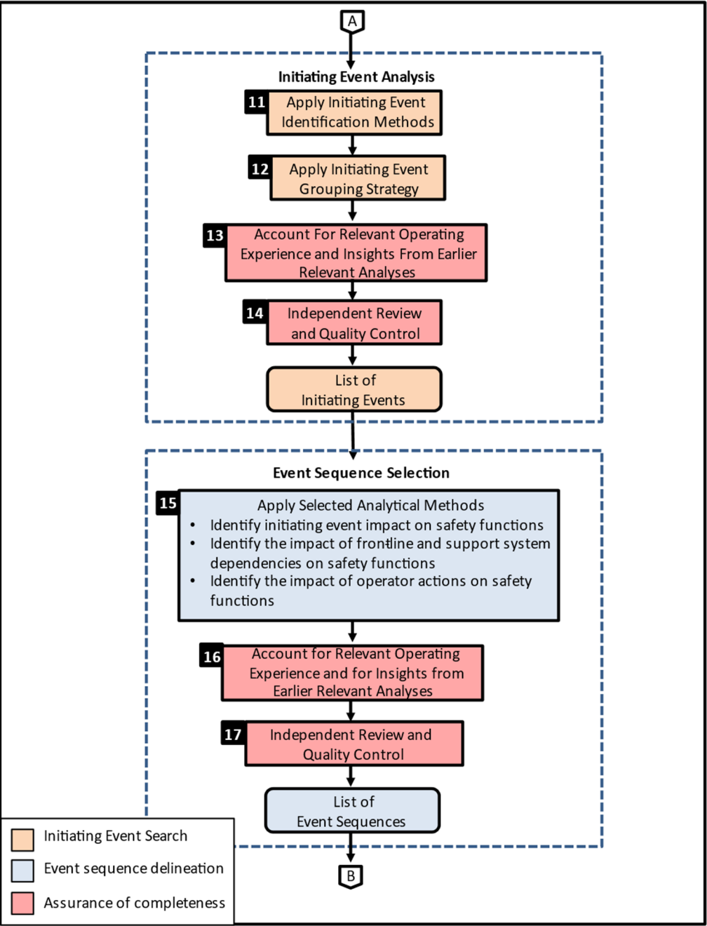
Figure 1. Technology-Inclusive Identification of Licensing Events (Sheet 2 of 3).
