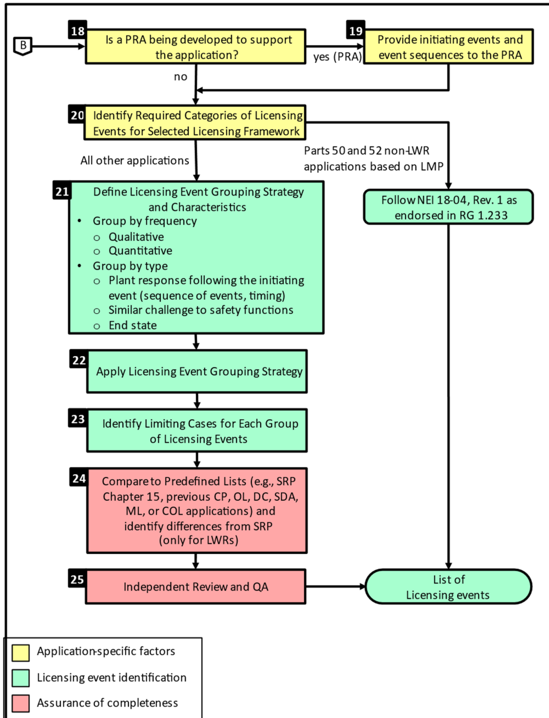
Figure 1. Technology-Inclusive Identification of Licensing Events (Sheet 3 of 3).
