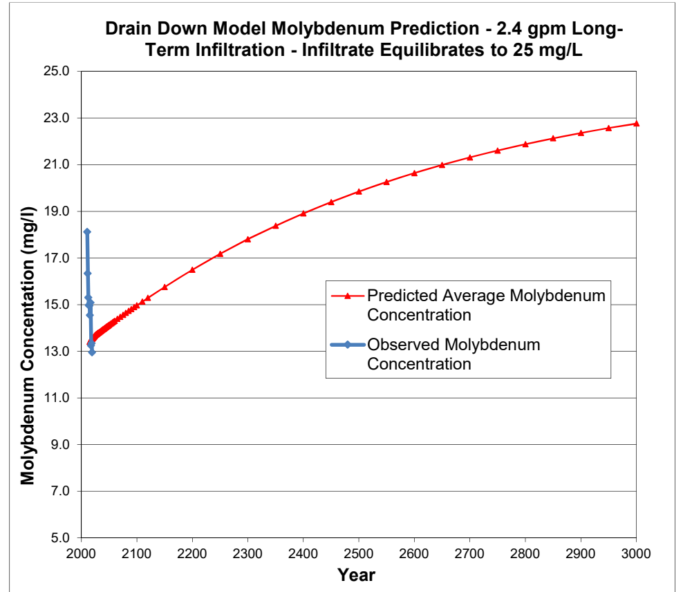
Figure 4 Drain Down Model Prediction with Infiltrate Equilibrating to 25 mg/L of Molybdenum Concentration 2.4 gpm Long-Term Infiltration Rate
