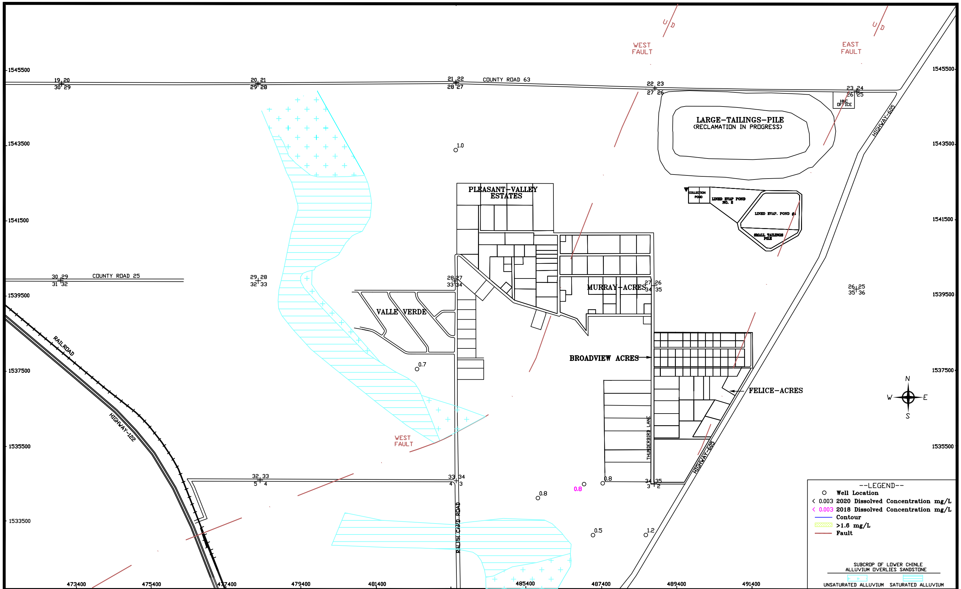
FLUORIDE CONCENTRATIONS OF THE LOWER CHINLE, 2020
