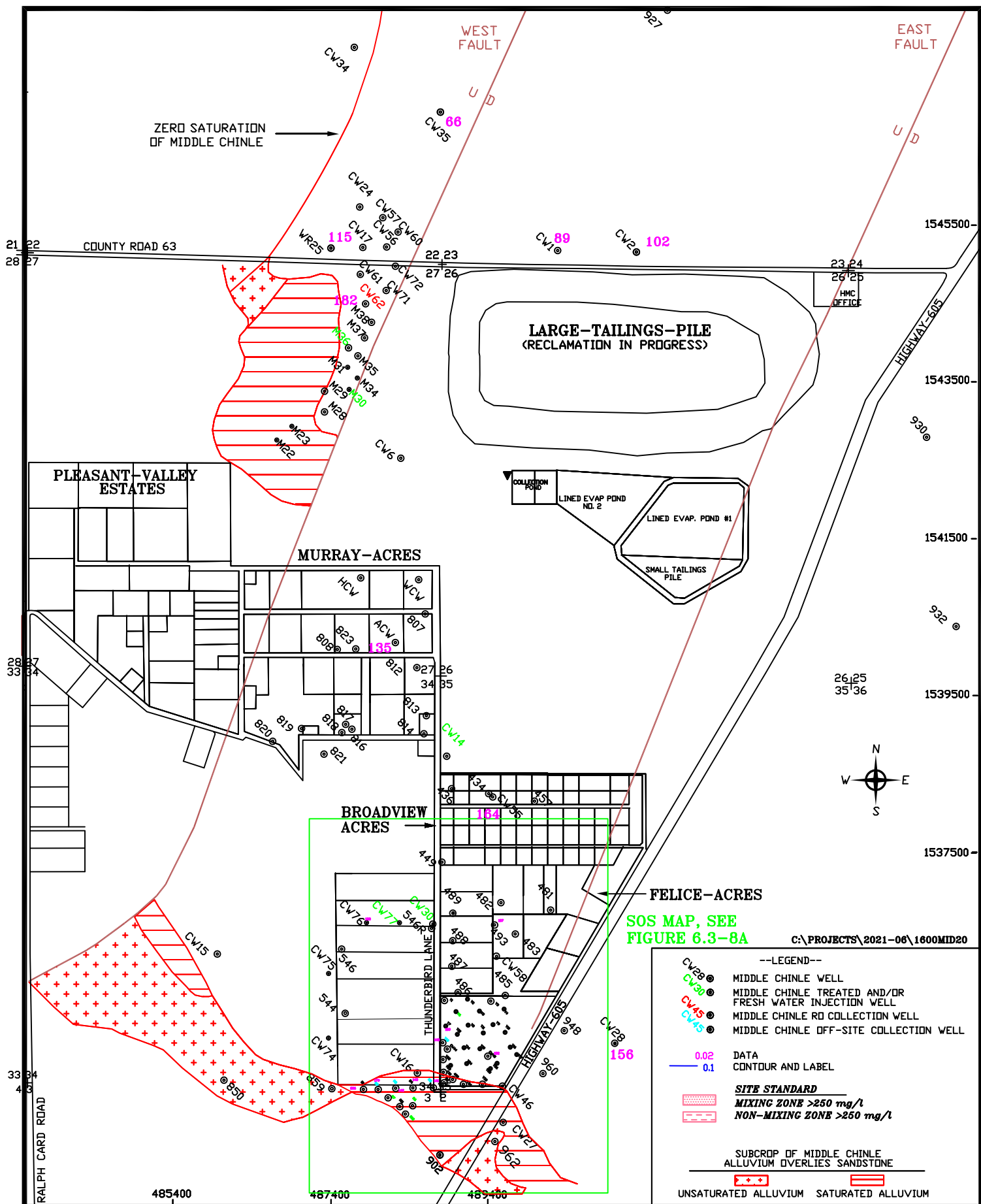
FIGURE 6.3-8. CHLORIDE CONCENTRATIONS OF THE MIDDLE CHINLE AQUIFER, 2020, mg/L
