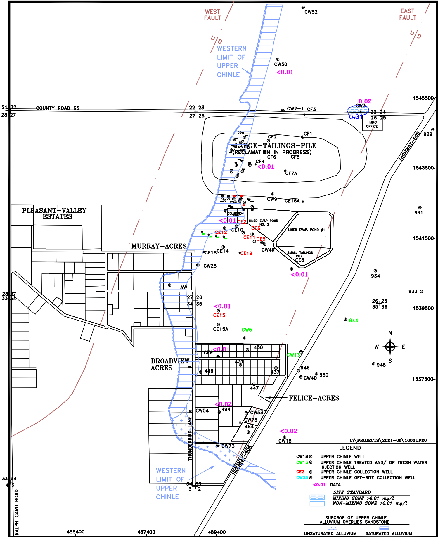
FIGURE 5.3-22. VANADIUM CONCENTRATIONS OF THE UPPER CHINLE AQUIFER, 2020, mg/L
