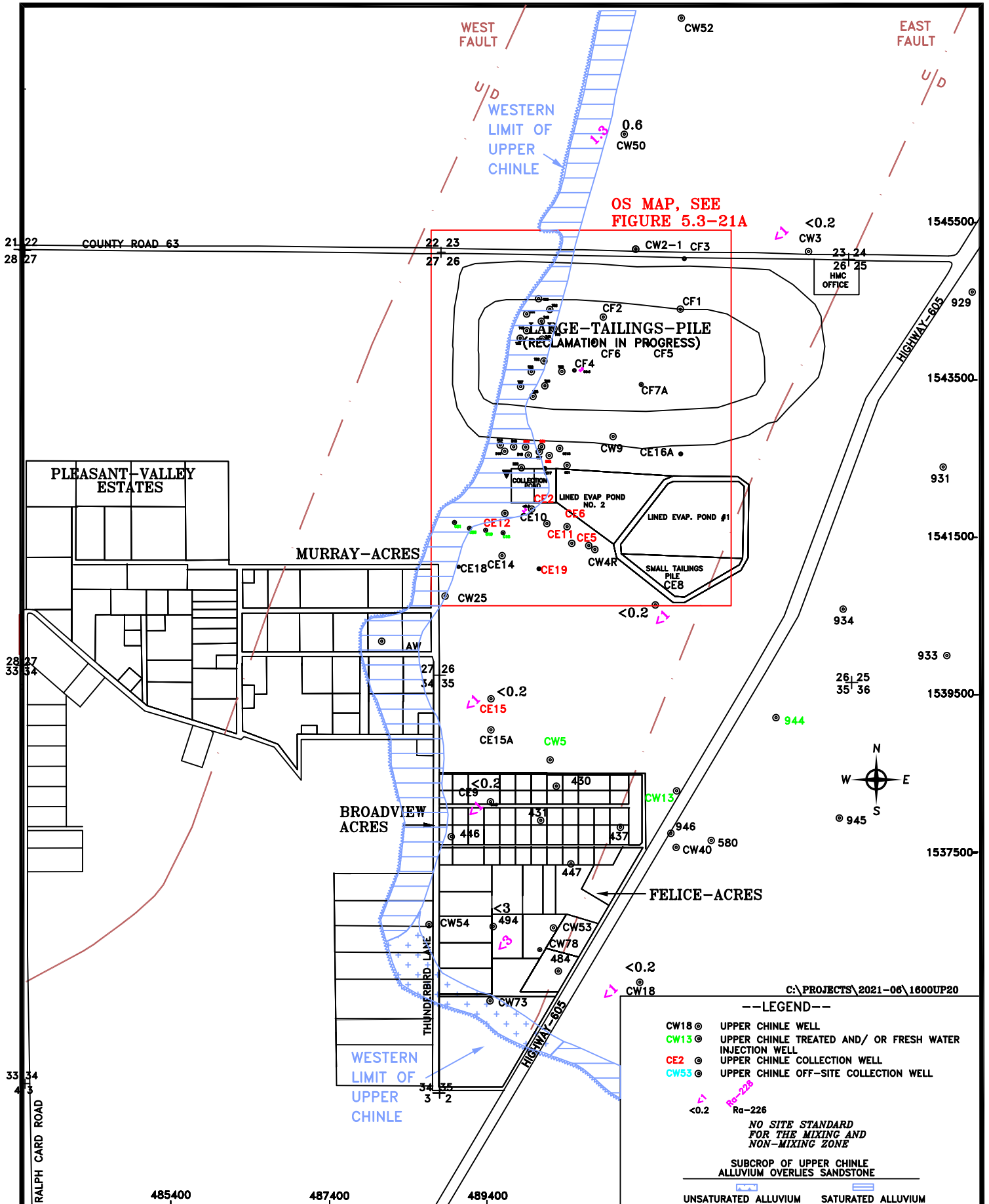
HOMESTAKE MILL AND ADJACENT PROPERTIES ~ GRANTS, NM ~ TOWNSHIP-11&12N, RANGE-10W FIGURE 5.3-21. RADIUM-226 AND RADIUM-228 CONCENTRATIONS OF THE UPPER CHINLE AQUIFER, 2020, pCi/L DATE: 12/9/2020 SCALE: 1" = 1600' PAGE: 5.3-36
