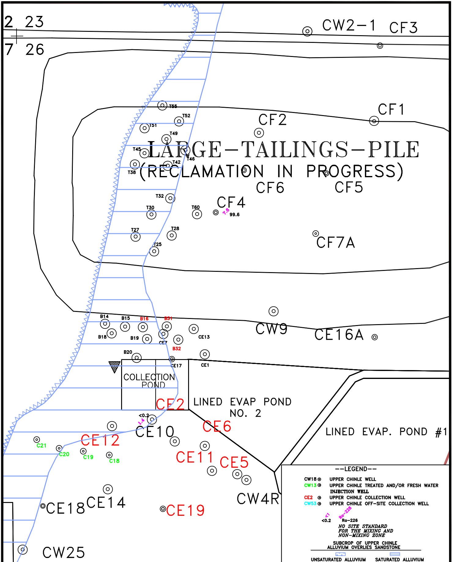
FIGURE 5.3-21A. RADIUM-226 AND RADIUM-228 CONCENTRATIONS OF THE UPPER CHINLE AQUIFER, OS, 2020, pCi/L
