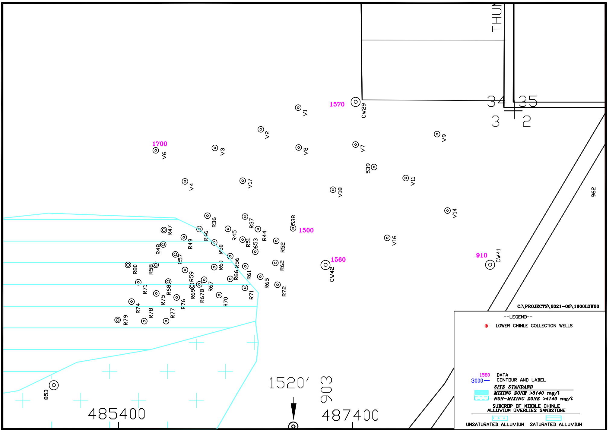
FIGURE 7.3-5A. TDS CONCENTRATIONS OF THE LOWER CHINLE AQUIFER, SOS, 2020, mg/L
