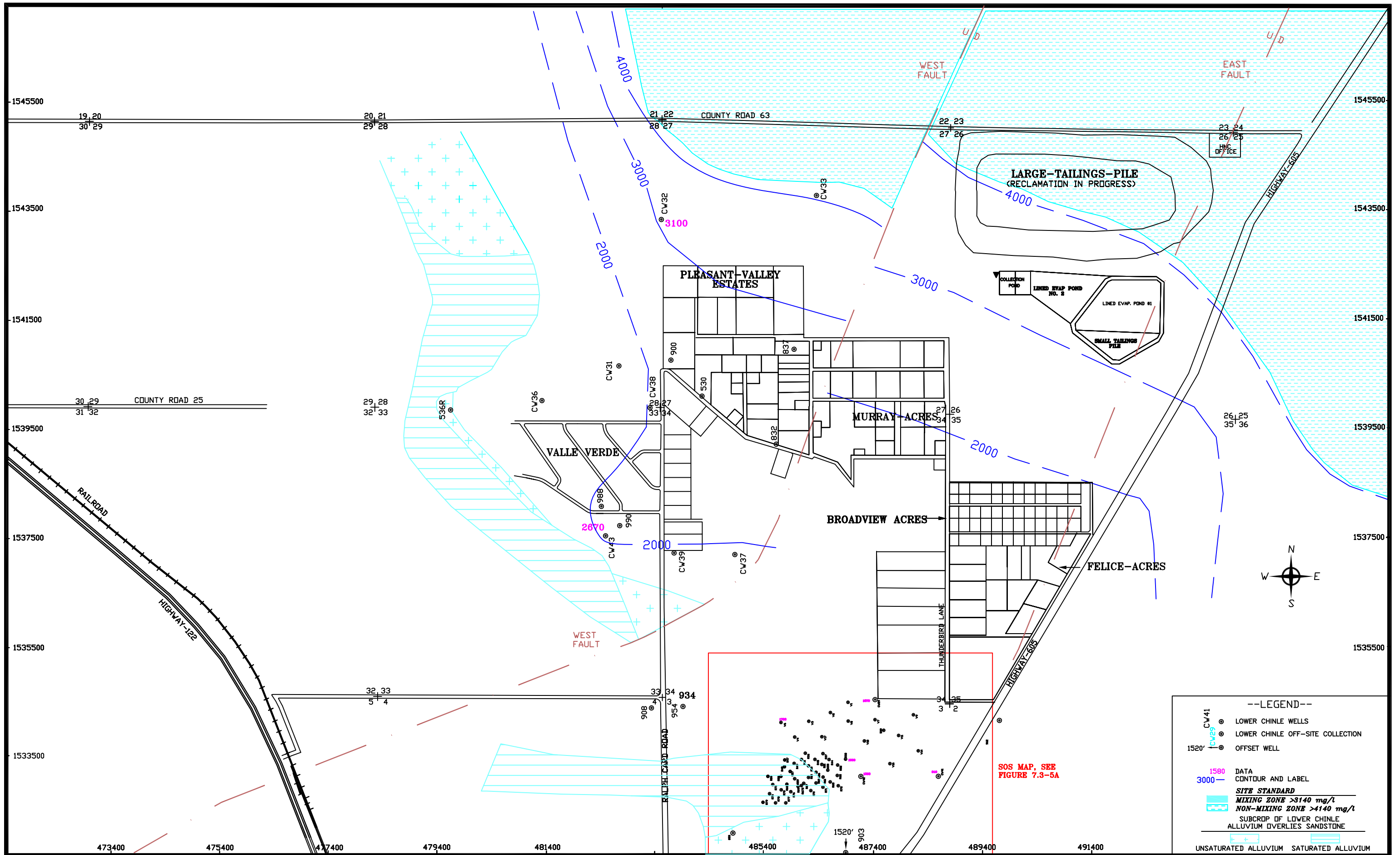
FIGURE 7.3-5. TDS CONCENTRATIONS OF THE LOWER CHINLE AQUIFER, 2020, mg/L PAGE 7.3-12
