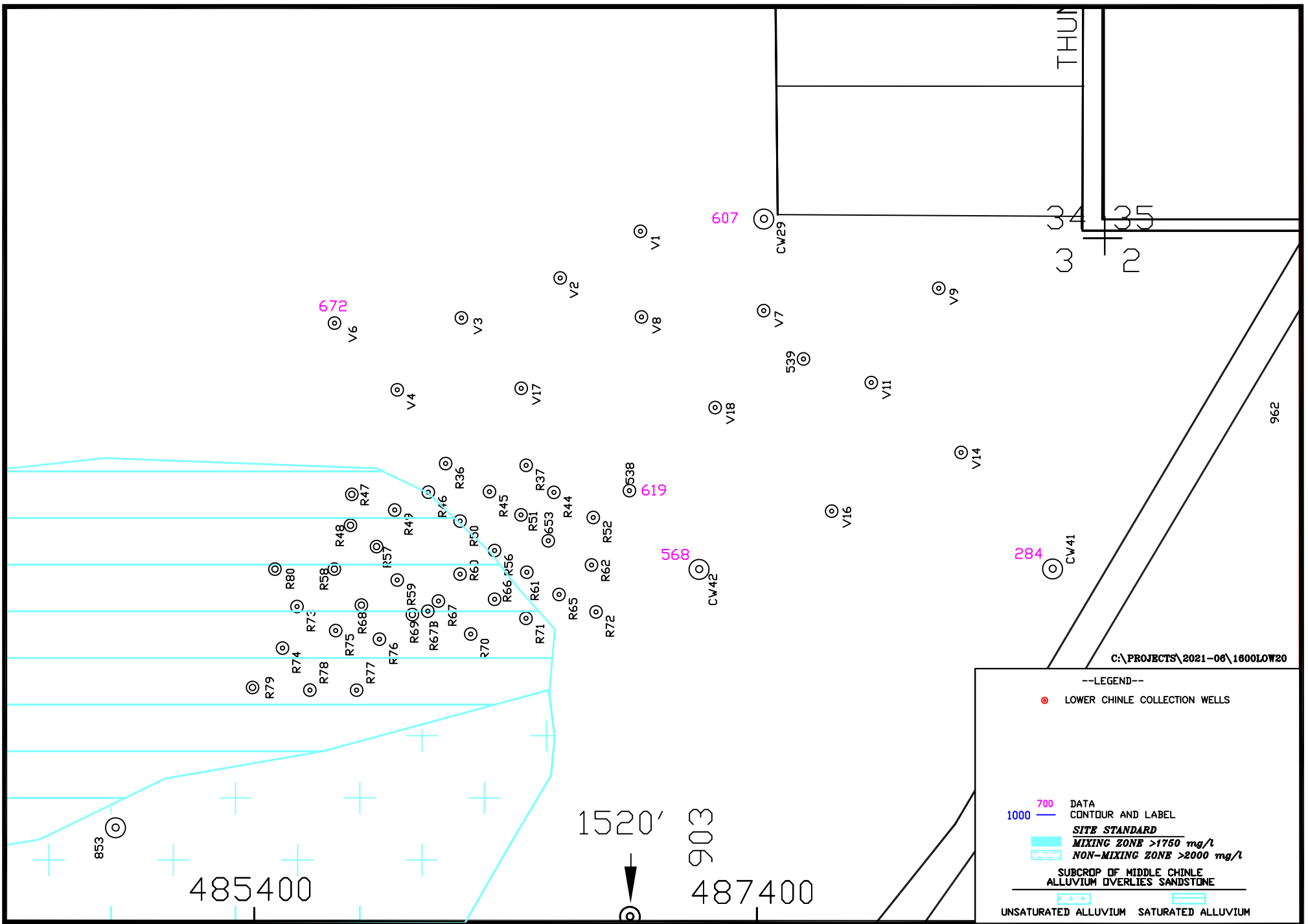
FIGURE 7.3-1B. SULFATE CONCENTRATIONS OF THE LOWER CHINLE AQUIFER, SOS, 2020, mg/L
