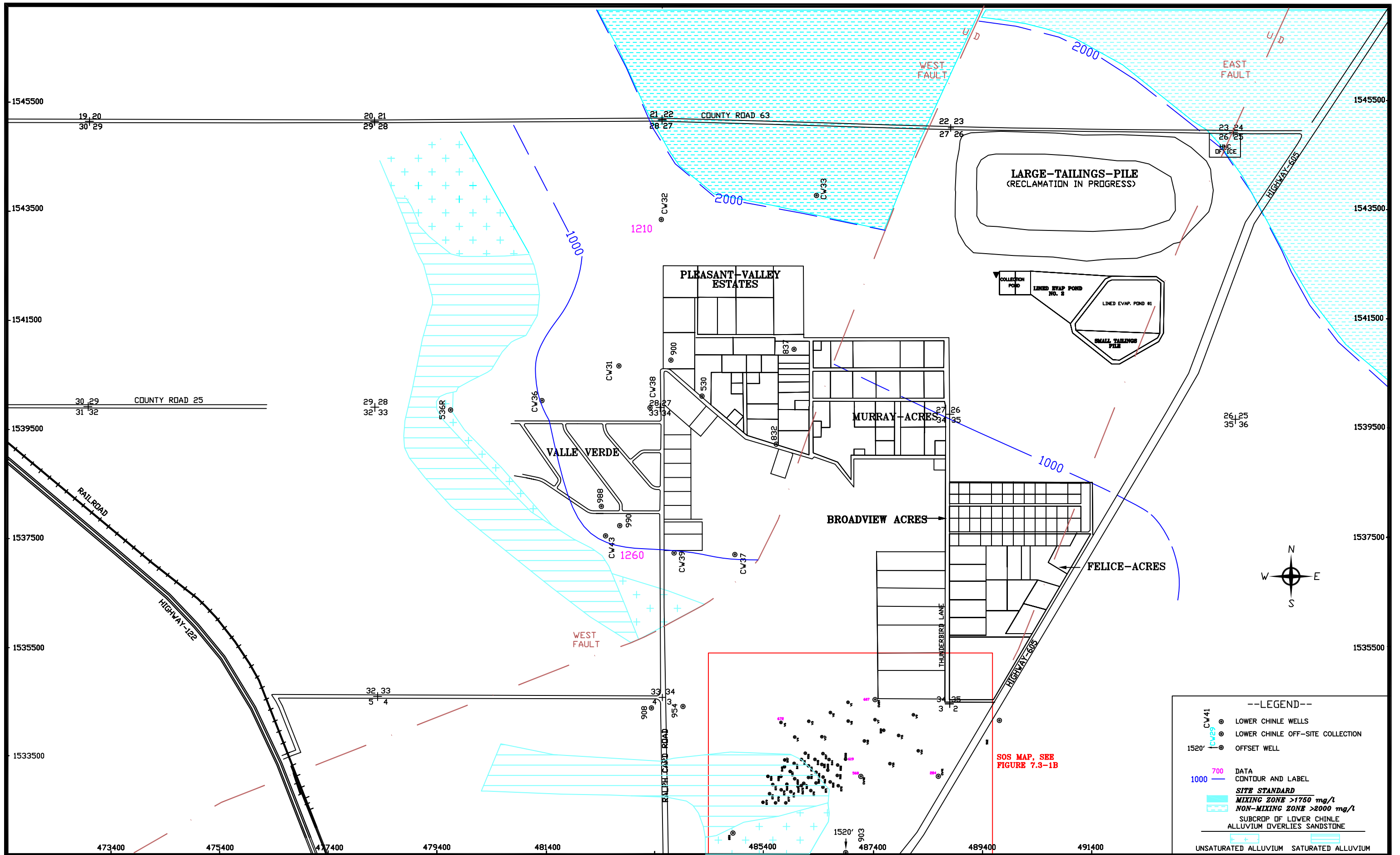
FIGURE 7.3-1A. SULFATE CONCENTRATIONS OF THE LOWER CHINLE AQUIFER, 2020, mg/L
