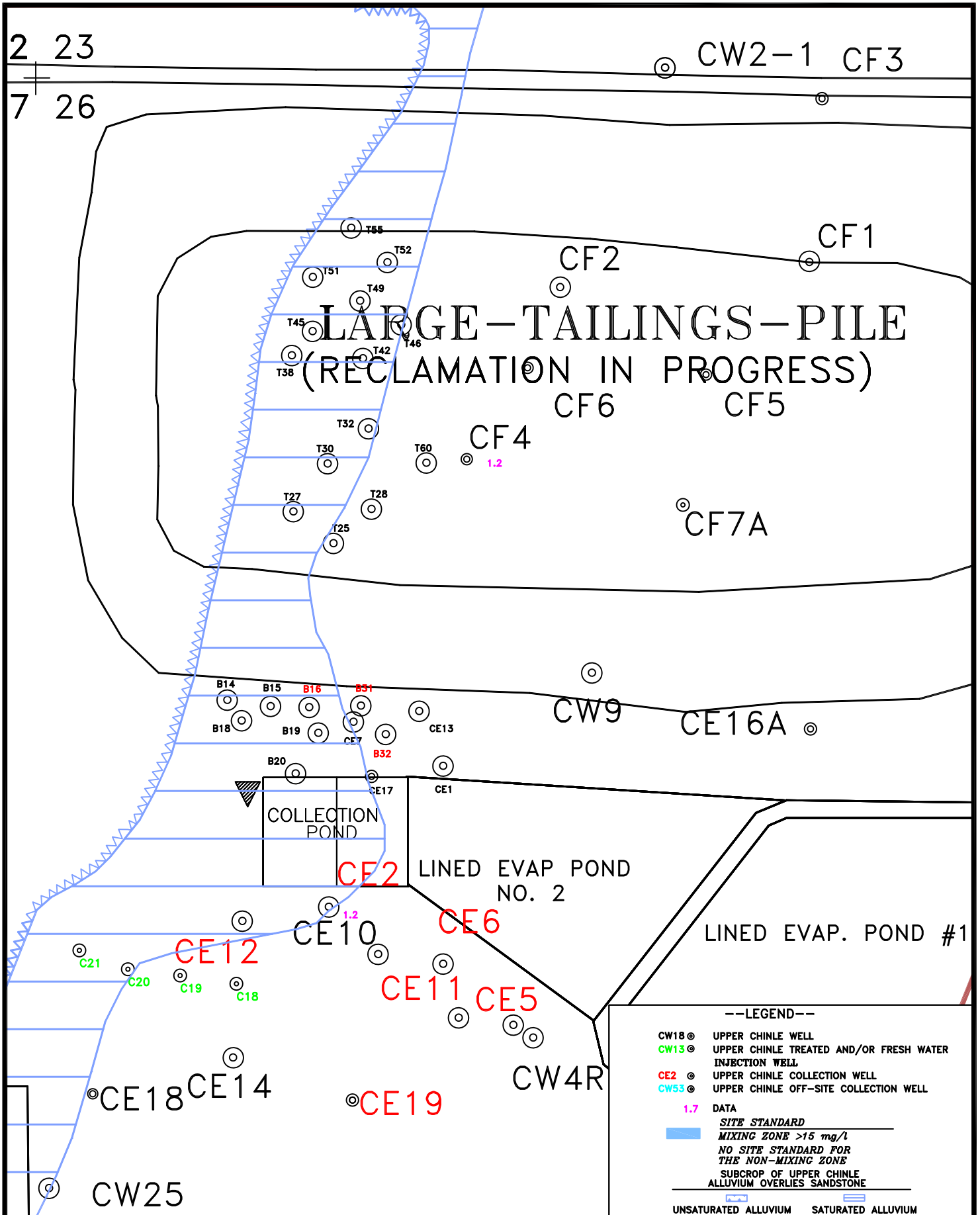
FIGURE 5.3-20A. NITRATE CONCENTRATIONS OF THE UPPER CHINLE AQUIFER, OS, 2020, mg/L
