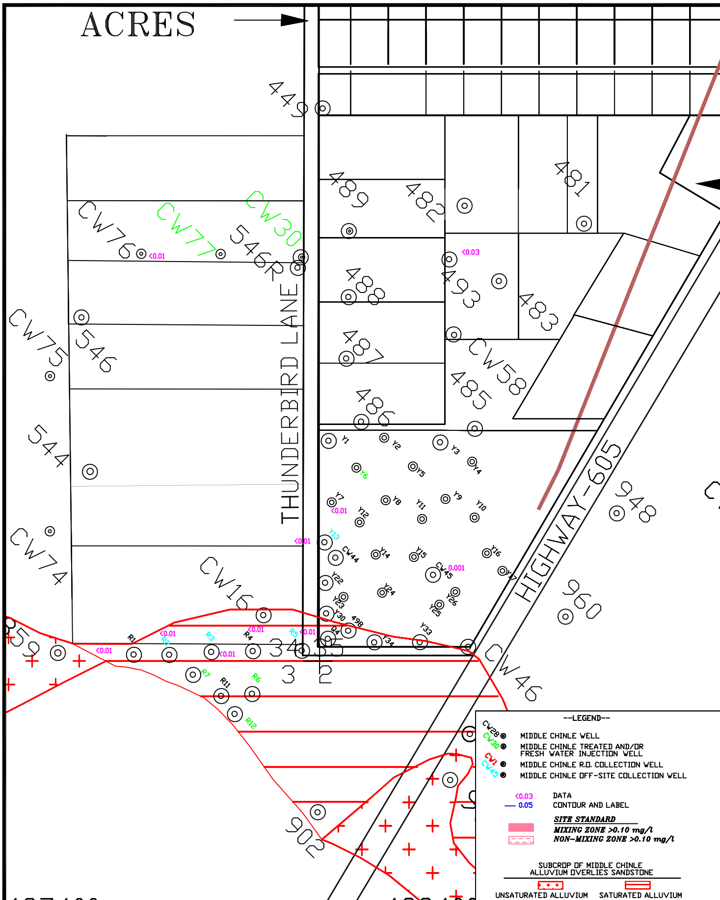
FIGURE 6.3-17A. MOLYBDENUM OF THE MIDDLE CHINLE AQUIFER, SOS, 2020, mg/L
