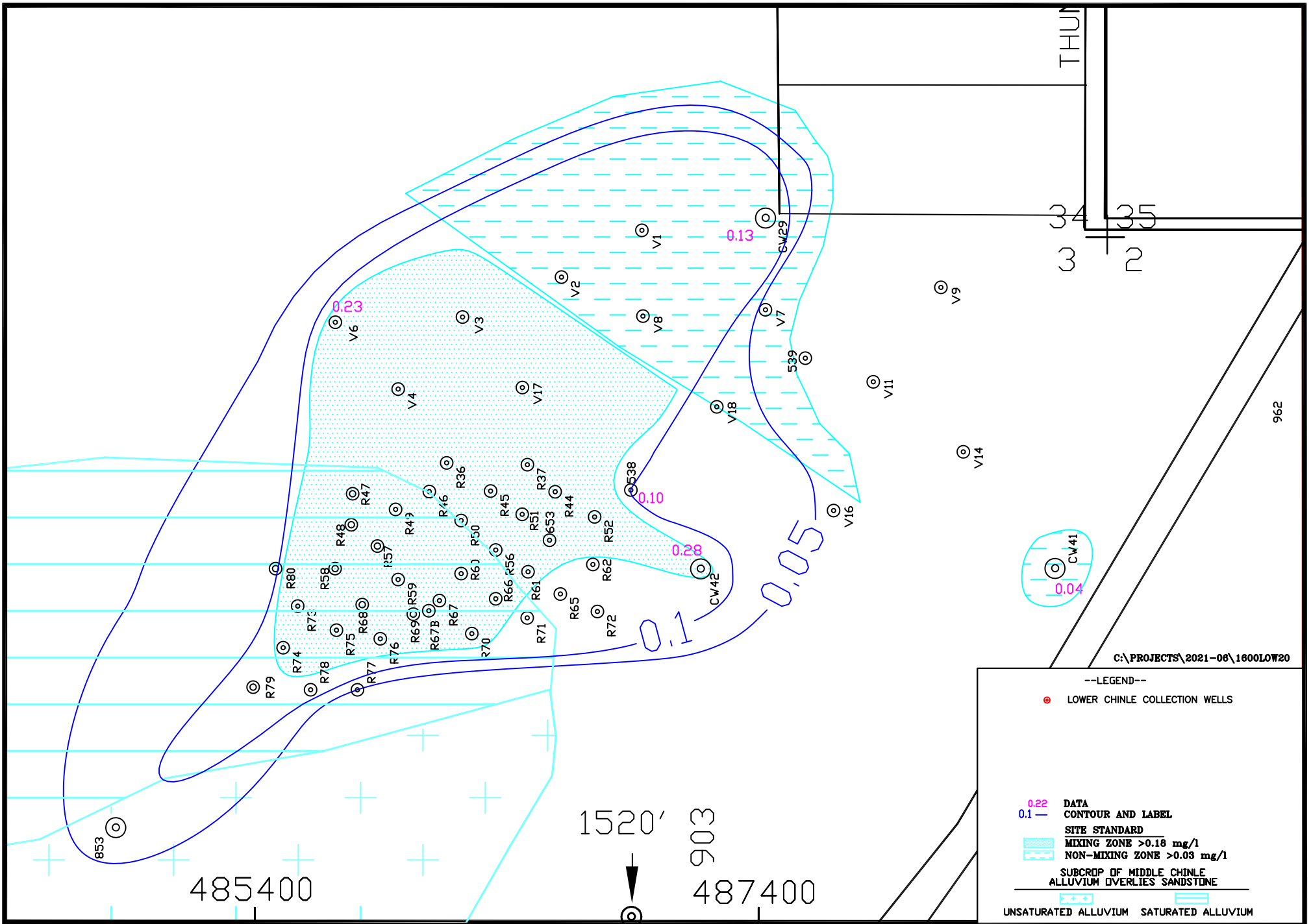
FIGURE 7.3-8A. URANIUM CONCENTRATIONS OF THE LOWER CHINLE AQUIFER, SOS, 2020, mg/L
