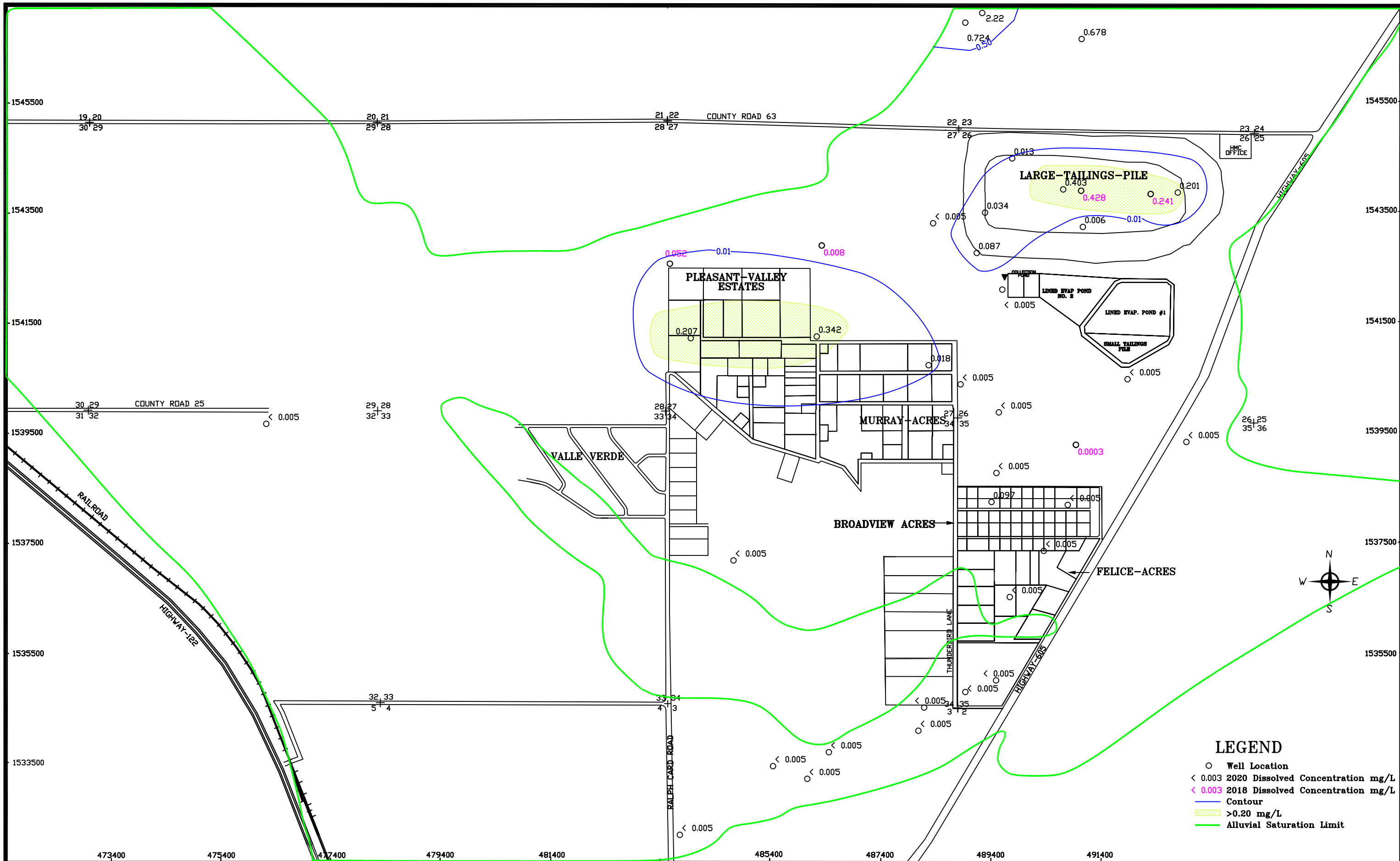
MANGANESE CONCENTRATIONS OF THE ALLUVIAL AQUIFER, 2020
