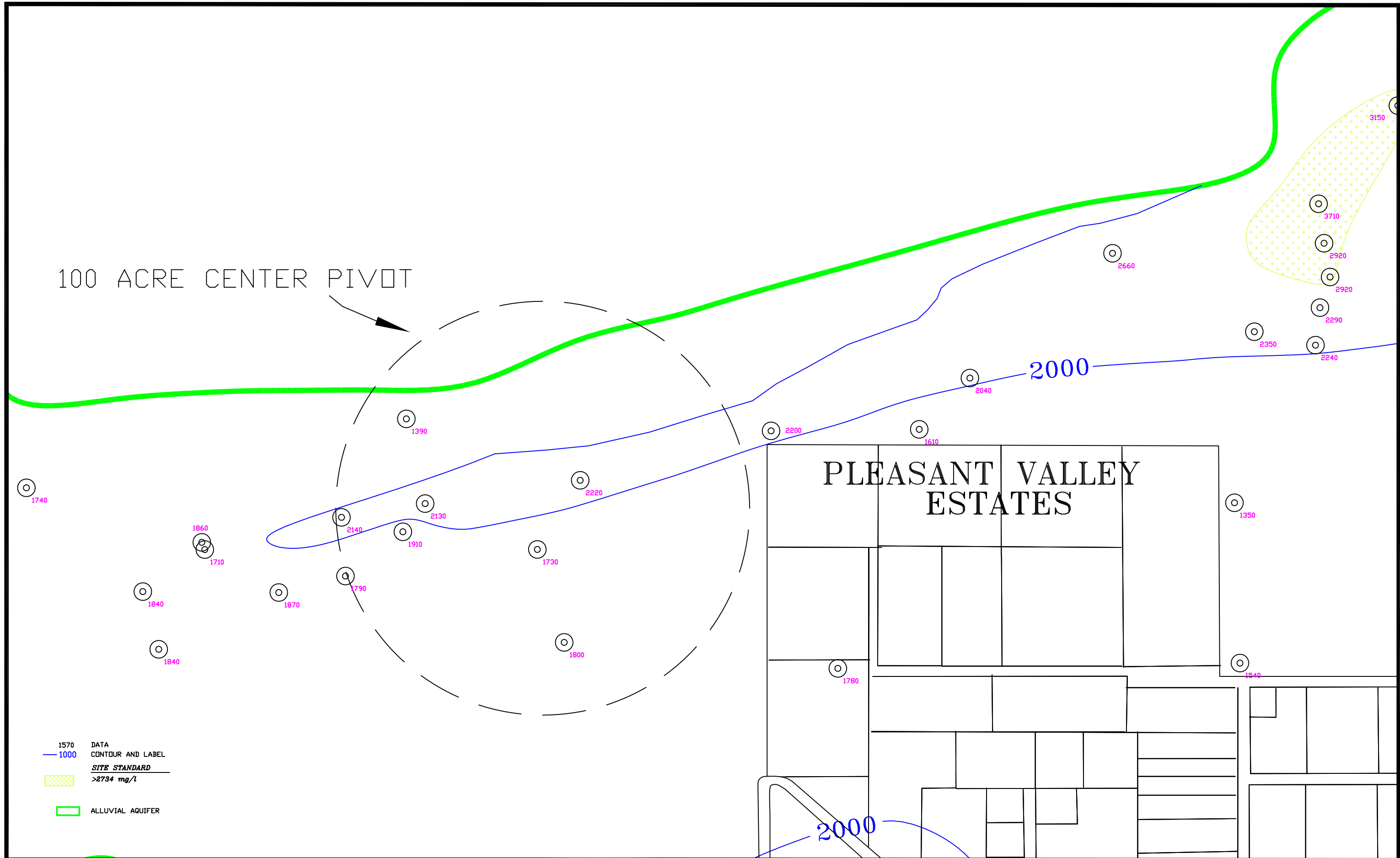
FIGURE 4.3-19C. TDS CONCENTRATIONS OF THE ALLUVIAL AQUIFER, NOS, 2020, mg/L 4.3-49
