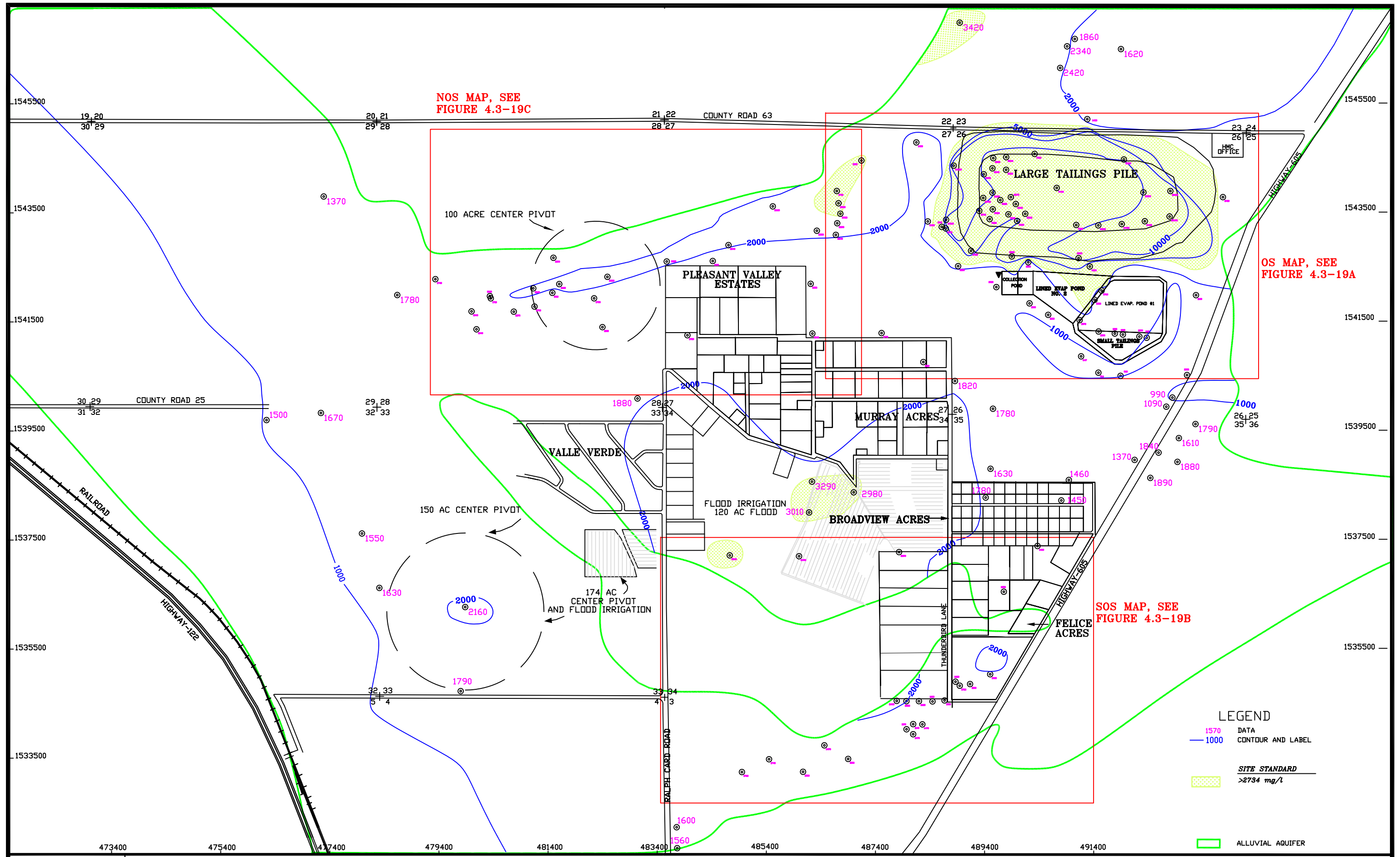
FIGURE 4.3-19. TDS CONCENTRATIONS OF THE ALLUVIAL AQUIFER, 2020, mg/L
