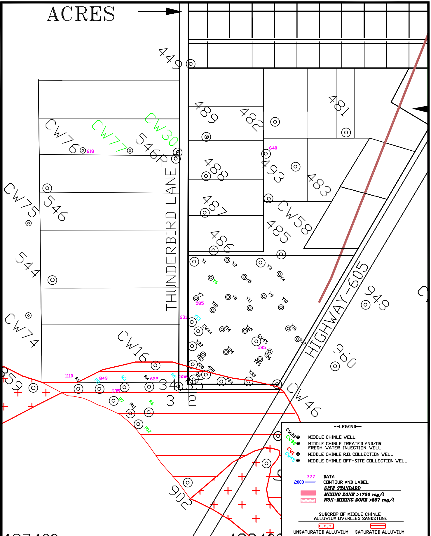
FIGURE 6.3-1B. SULFATE CONCENTRATIONS OF THE MIDDLE CHINLE AQUIFER, 2020, SOS, mg/L
