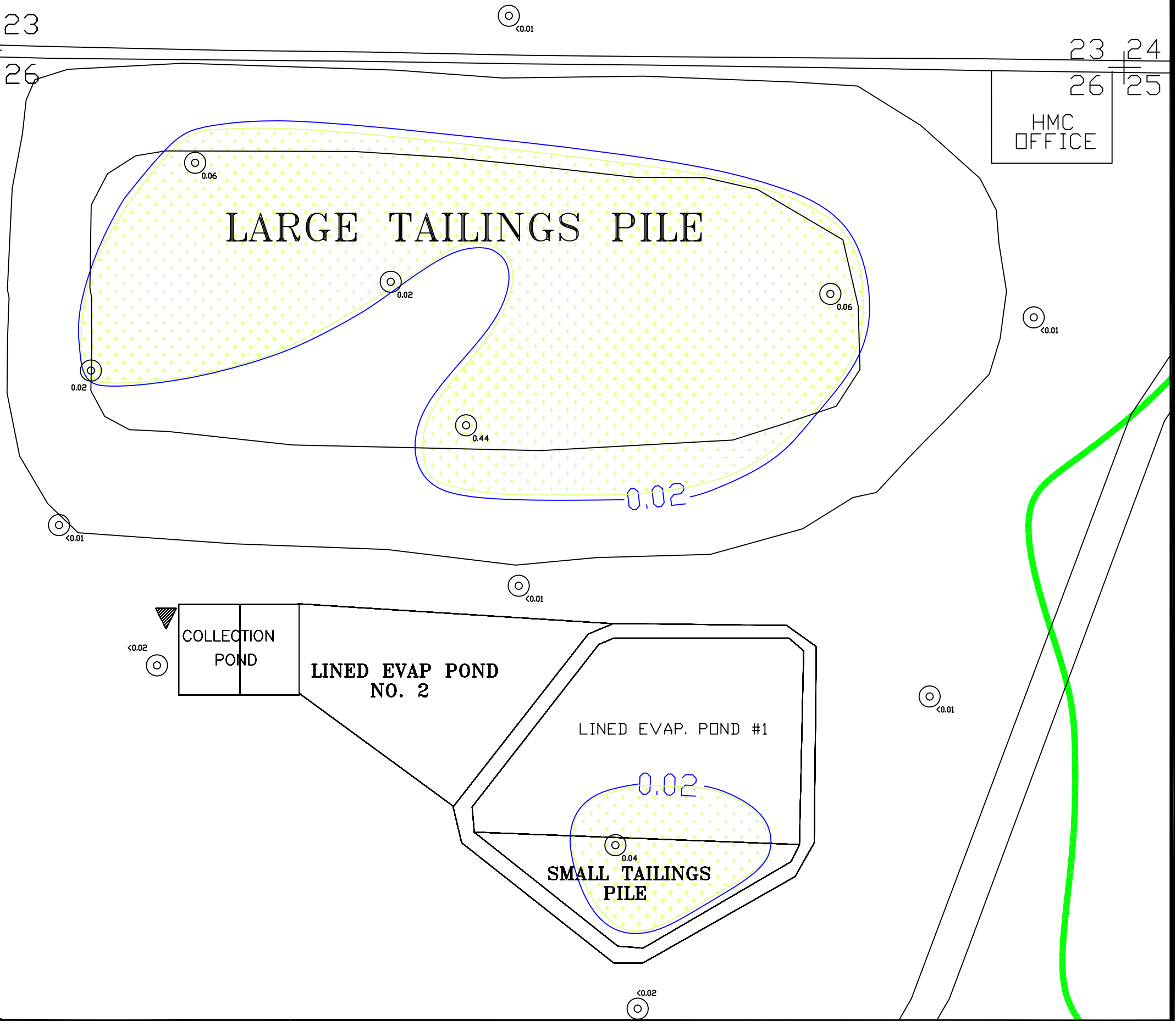
FIGURE 4.3-122A. VANADIUM CONCENTRATIONS OF THE ALLUVIAL AQUIFER, OS, 2020, mg/L 4.3-188
