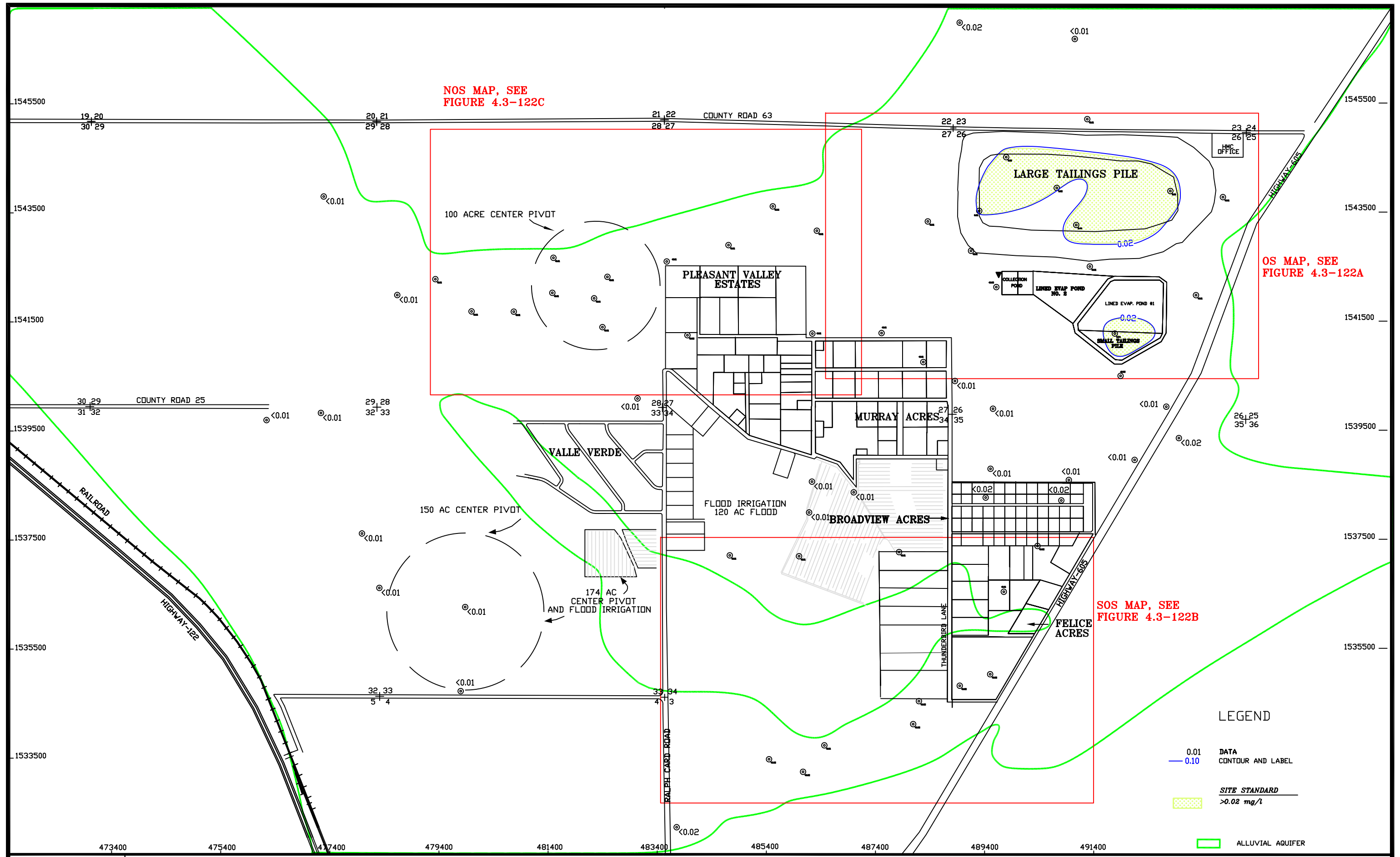
FIGURE 4.3-122. VANADIUM CONCENTRATIONS OF THE ALLUVIAL AQUIFER, 2020, mg/L
