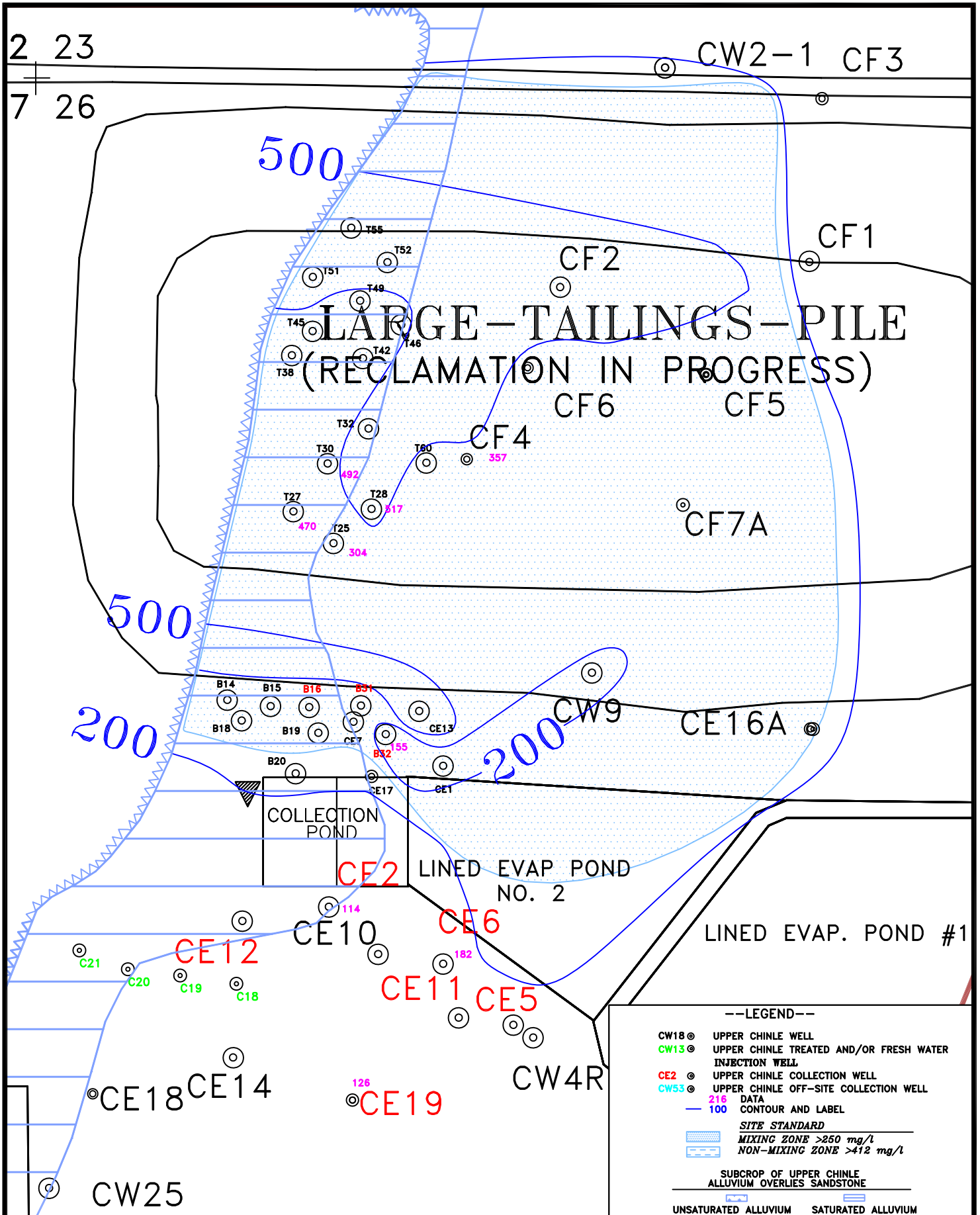
HOMESTAKE MILL AND ADJACENT PROPERTIES ~ GRANTS, NM ~ TOWNSHIP-11&12N, RANGE-10W DATE: 1/18/2021 SCALE: 1" = 500' FIGURE 5.3-8A. CHLORIDE CONCENTRATIONS OF THE UPPER CHINLE AQUIFER, OS, 2020, mg/L PAGE: 5.3-19
