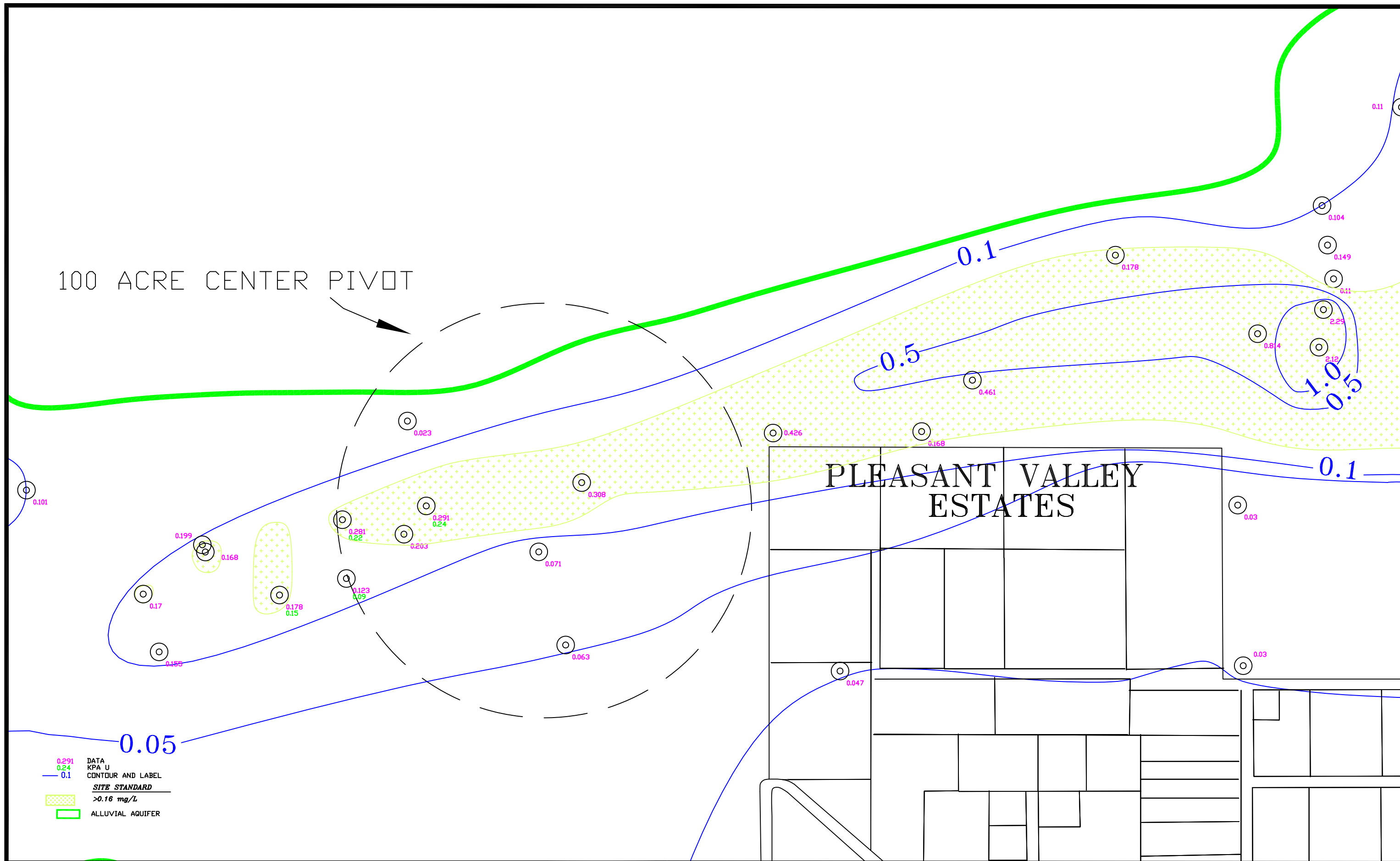
FIGURE 4.3-53C. URANIUM CONCENTRATIONS OF THE ALLUVIAL AQUIFER, NOS, 2020, mg/L 4.3-95
