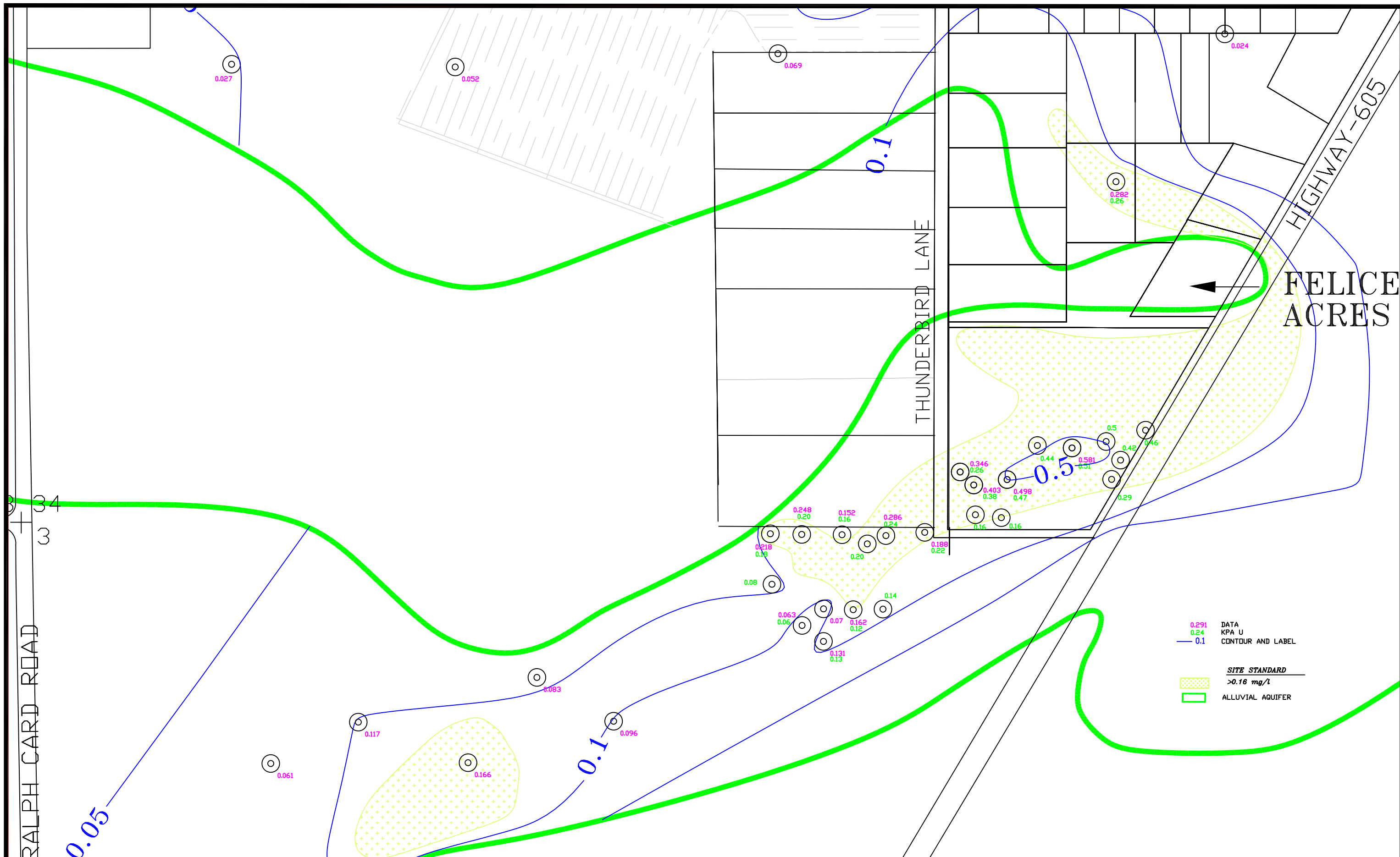
FIGURE 4.3-53B. URANIUM CONCENTRATIONS OF THE ALLUVIAL AQUIFER, SOS, 2020, mg/L 4.3-94
