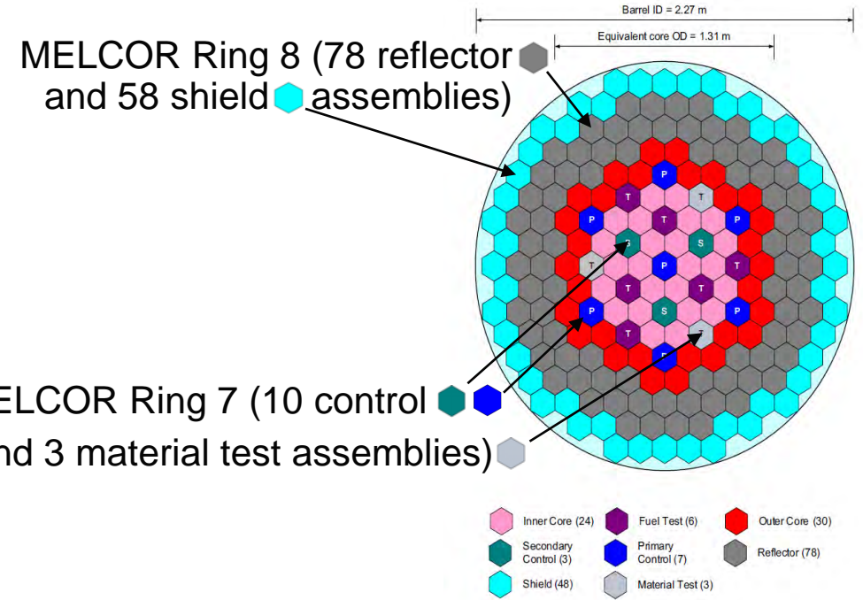
Figure II.1-1 Reference ABTR Core Configuration
