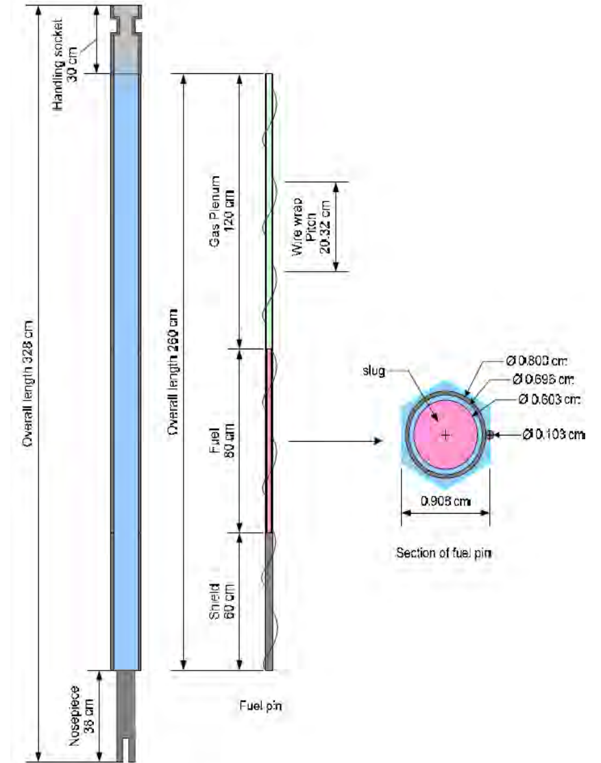
ABTR Fuel [ANL-AFCI-173]
