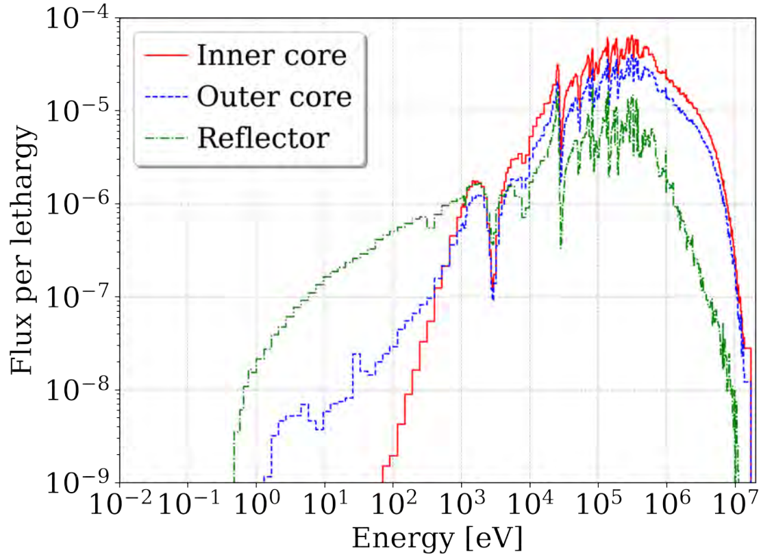
Energy-dependent Flux Spectrum
