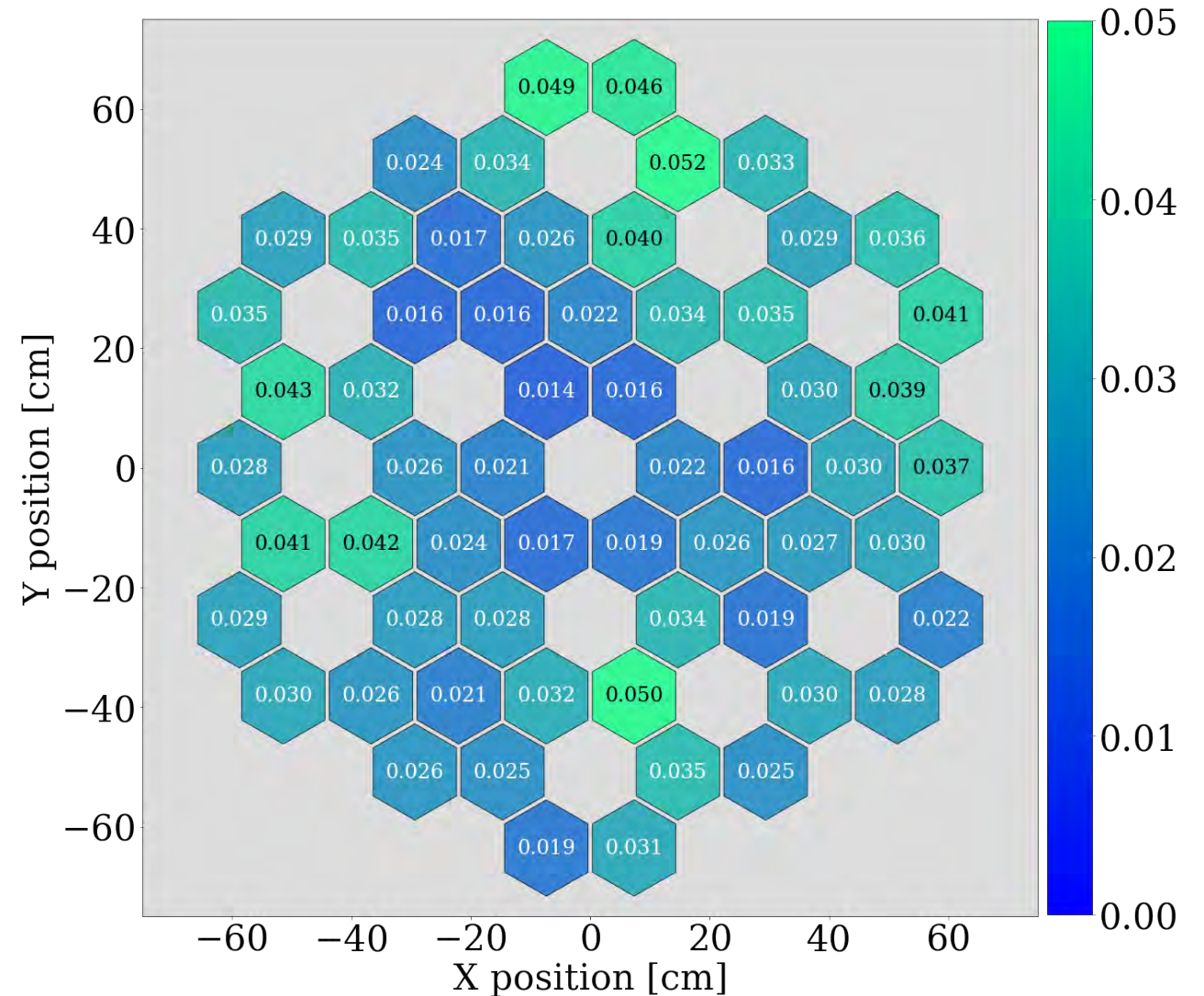
Statistical error (%) in assembly power
