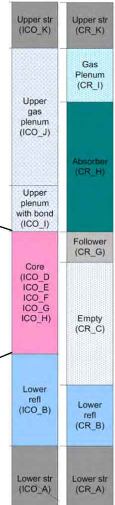
Fuel and Control Assembly Cross Section [2]
