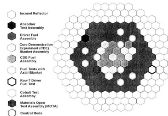
FFTF Reactor Core and Vessel
