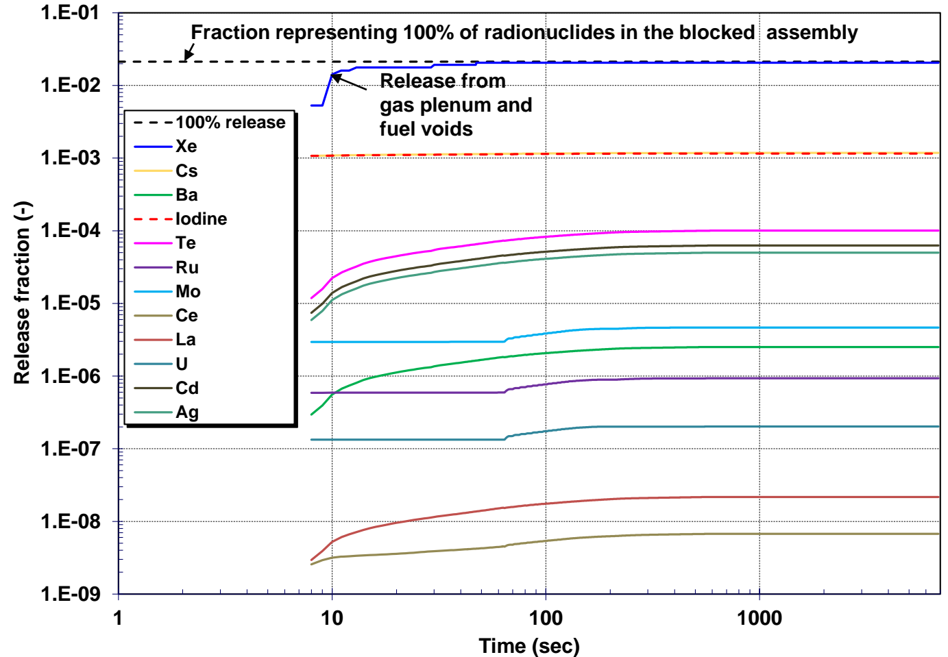
Radionuclide release fraction from the fuel based on whole core inventory
