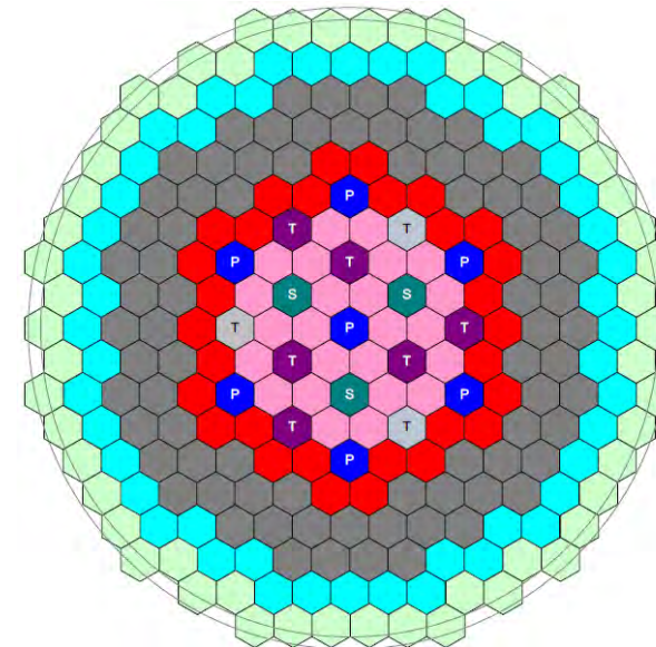
ABTR Core [2]
