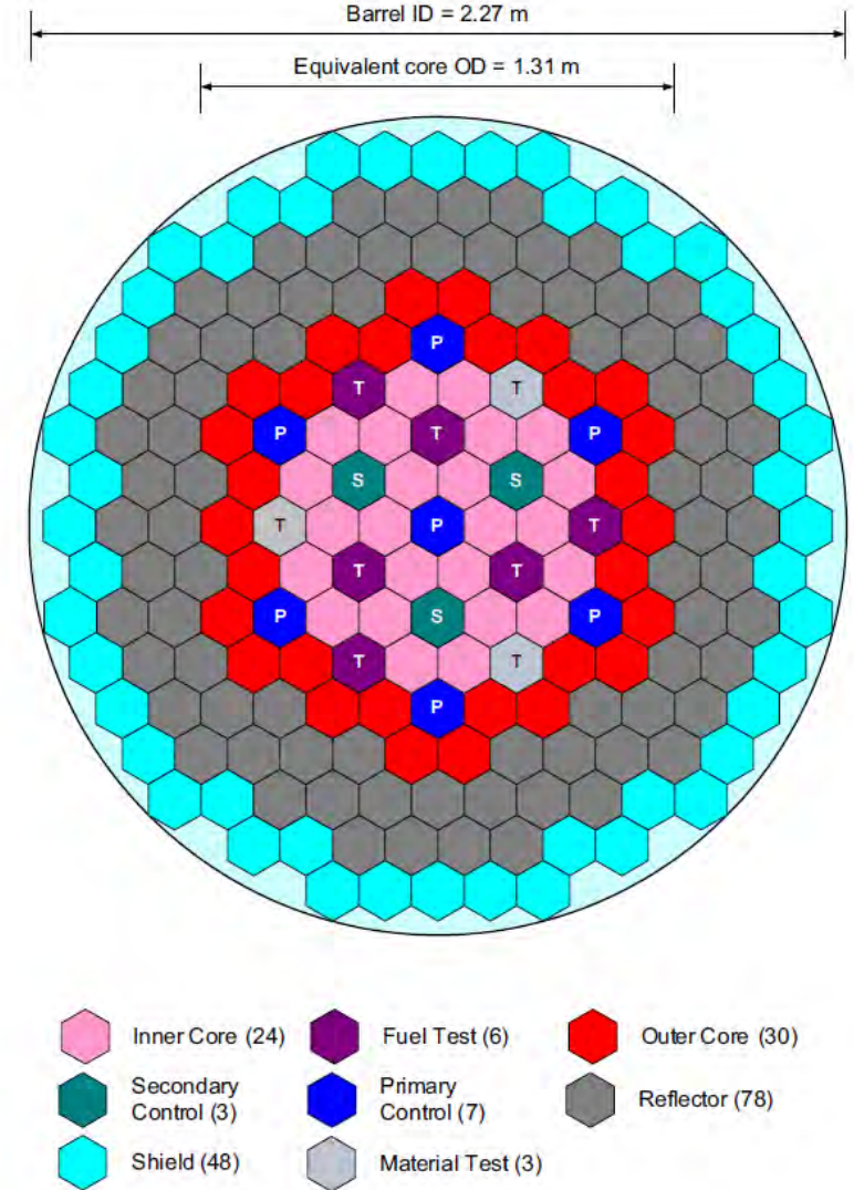
Figure II.1-1 Reference ABTR Core Configuration
