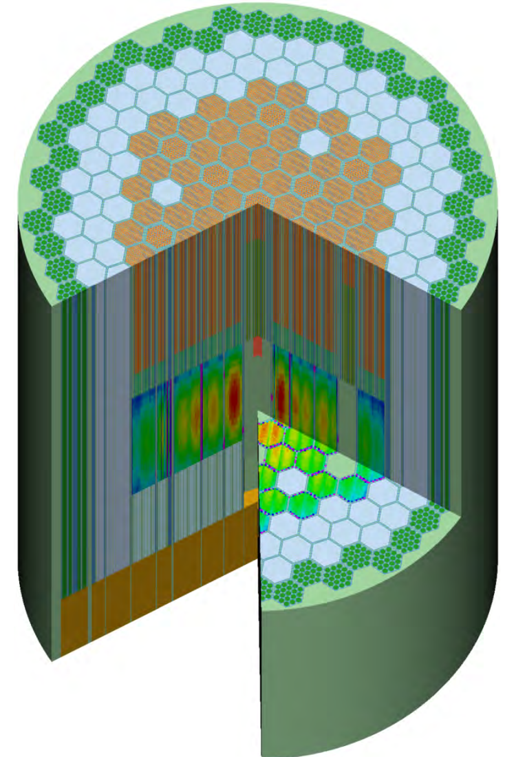
3D SCALE ABTR Core with Fission Density Overlay
