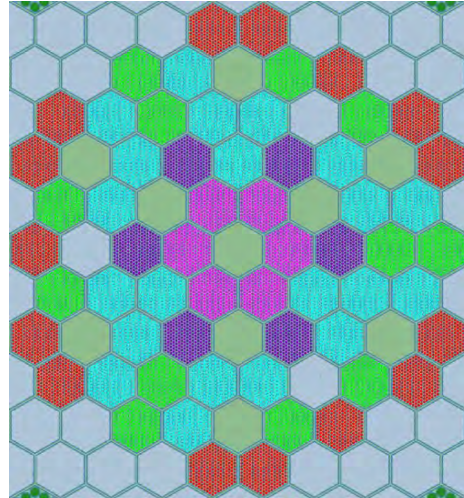
ABTR Model with Color-Coded Assemblies
