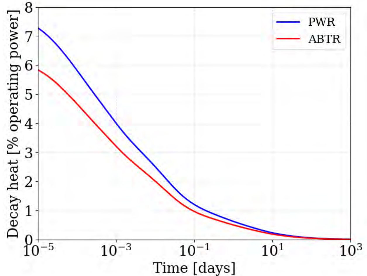
Total decay heat after shutdown
