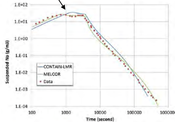
Figure 33. Suspended Na Aerosol Mass - AB1
