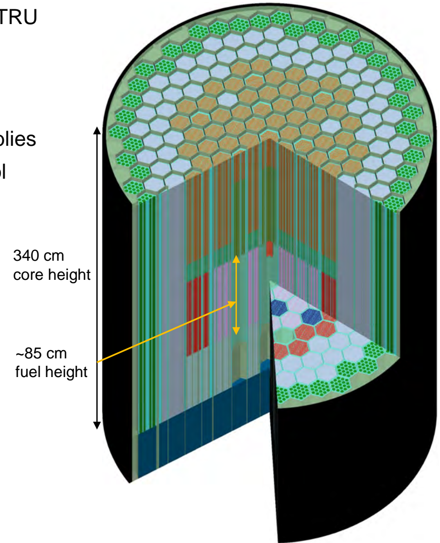
3D SCALE Model
