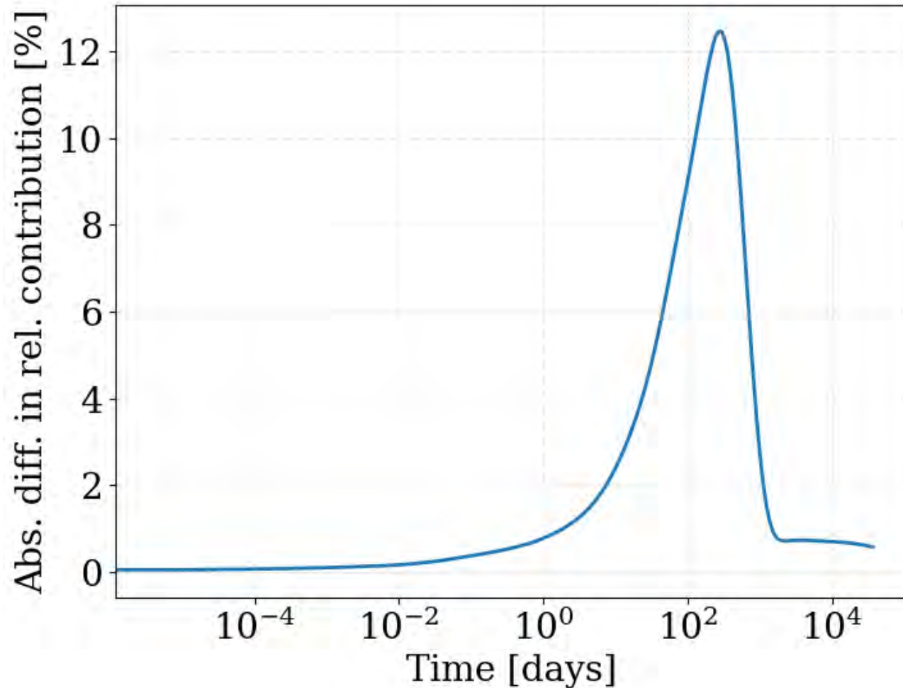
Difference in Cm-242 contribution to decay heat between ABTR and PWR
