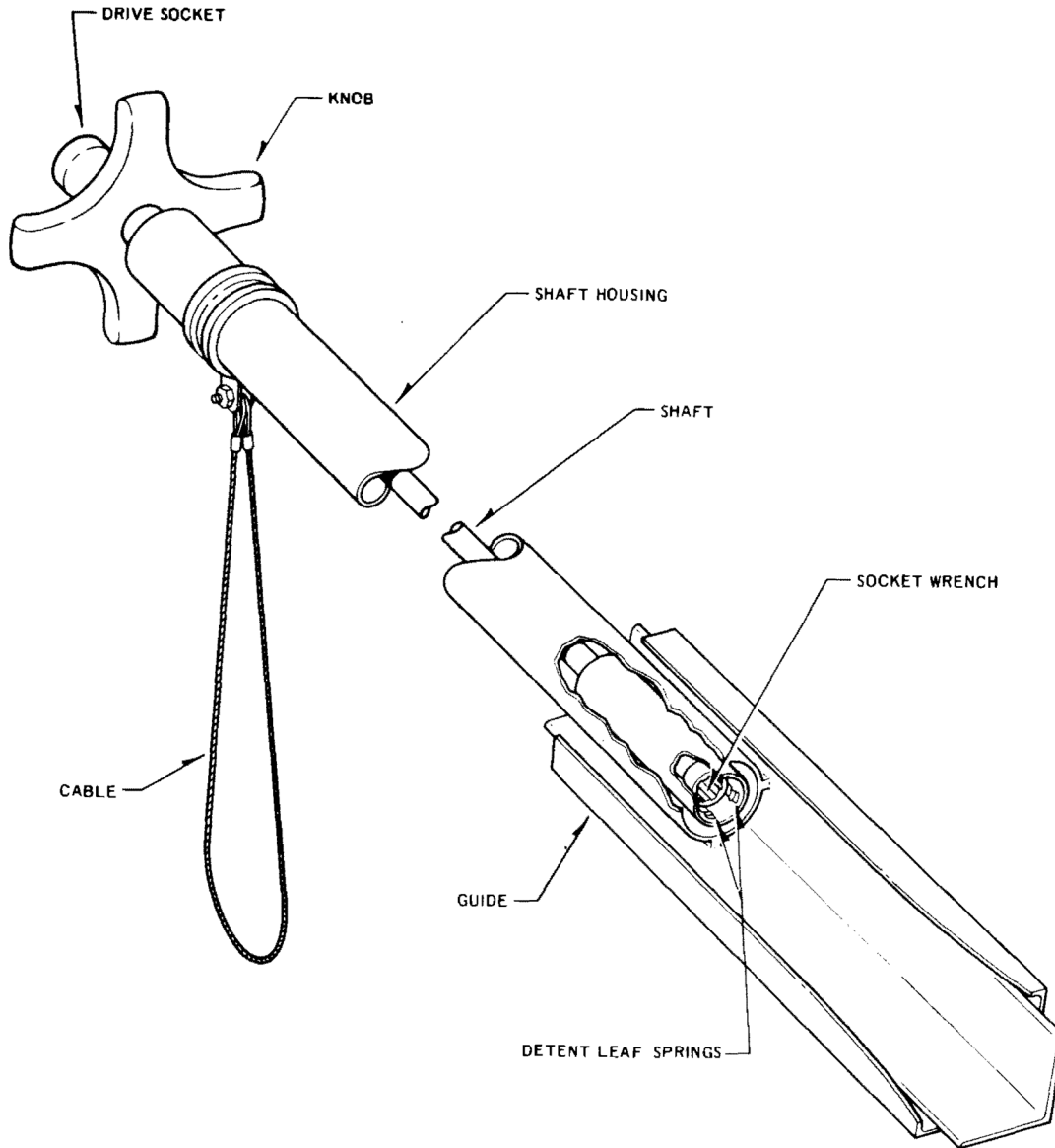
MISSISSIPPI POWER & LIGHT COMPANY GRAND GULF NUCLEAR STATION UNITS 1 & 2 UPDATED FINAL SAFETY ANALYSIS REPORT CHANNEL BOLT WRENCH FIGURE 9.1-8
