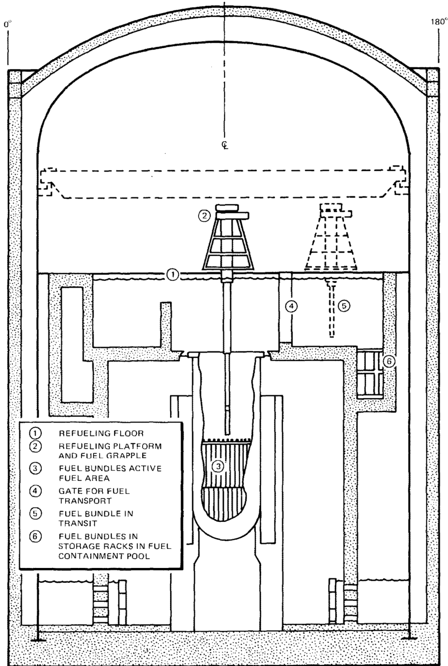
MISSISSIPPI POWER & LIGHT COMPANY GRAND GULF NUCLEAR STATION UNITS 1 & 2 UPDATED FINAL SAFETY ANALYSIS REPORT FUEL BUNDLE TRANSFER SEQUENCE GE STANDARD PLANT FIGURE 9.1-22
