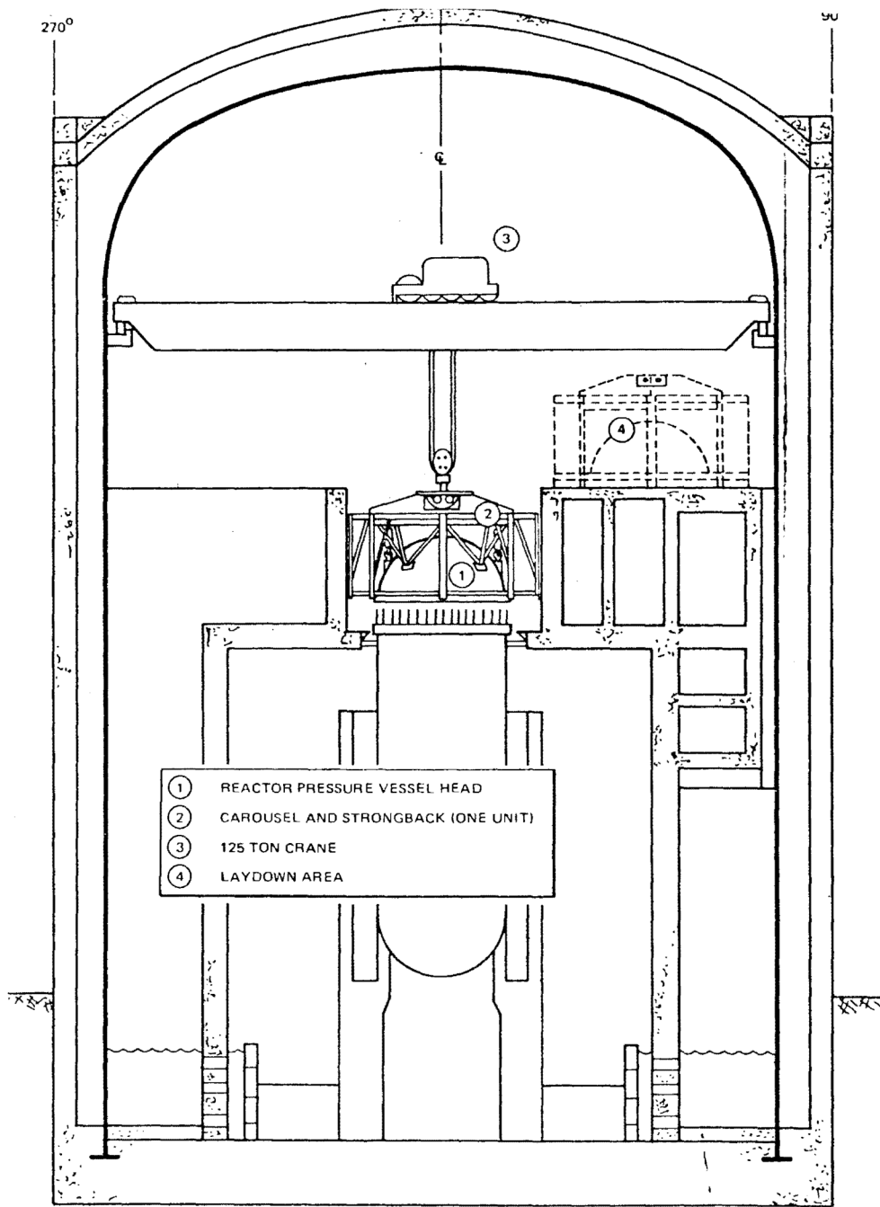
MISSISSIPPI POWER & LIGHT COMPANY GRAND GULF NUCLEAR STATION UNITS 1 & 2 UPDATED FINAL SAFETY ANALYSIS REPORT REACTOR VESSEL HEAD REMOVAL SEQUENCE GE STANDARD PLANT FIGURE 9.1-19
