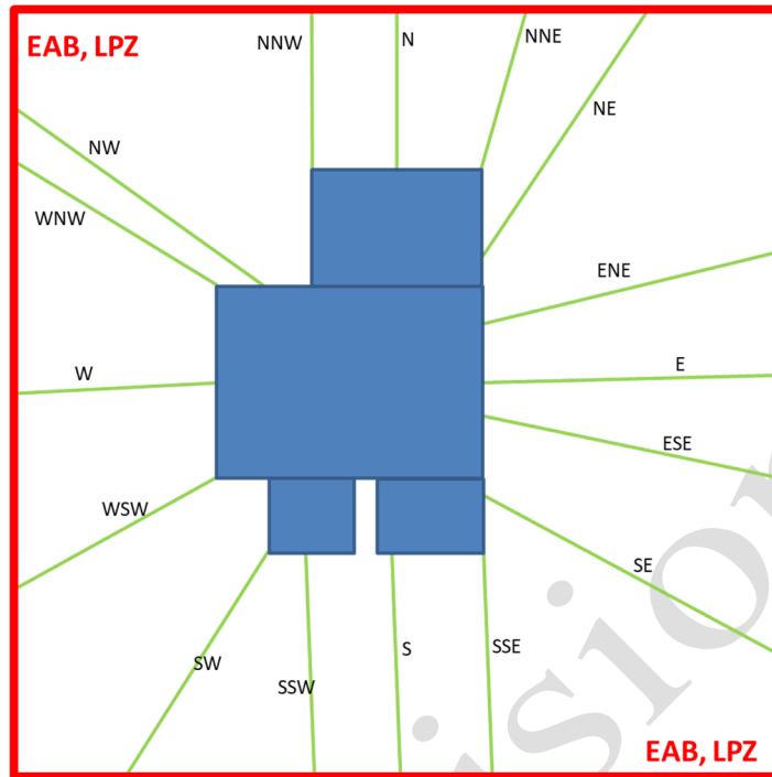
Figure 2-2 Example of how to use the closest point of a building withing each of the 16 directional sectors from the nuclear island to the EAB/LPZ boundaries
