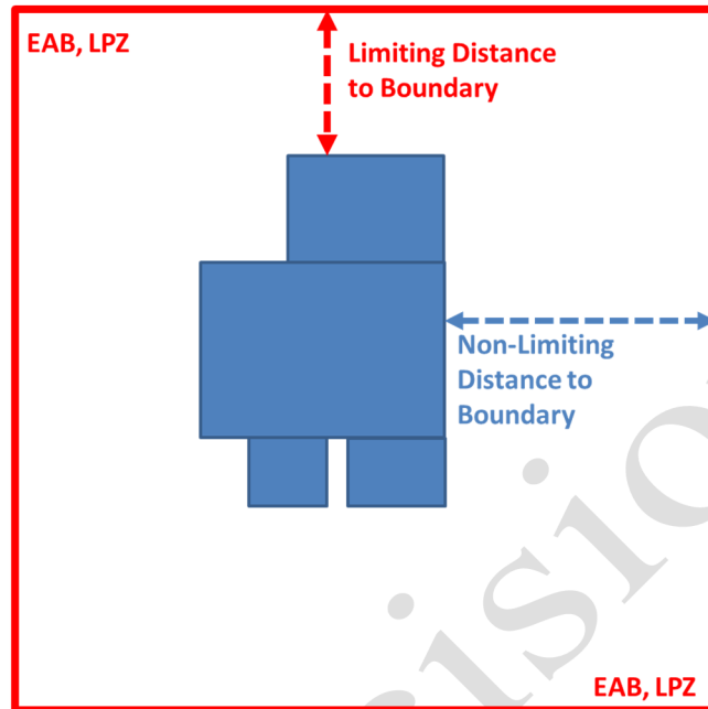
Figure 2-1 Example of limiting and nonlimiting distances from buildings within the nuclear island to the EAB/LPZ boundaries
