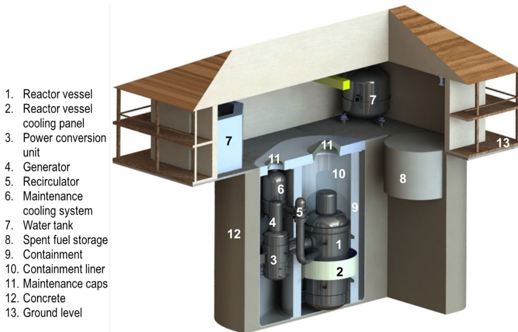
Figure 1. FMR Nuclear Island Components
