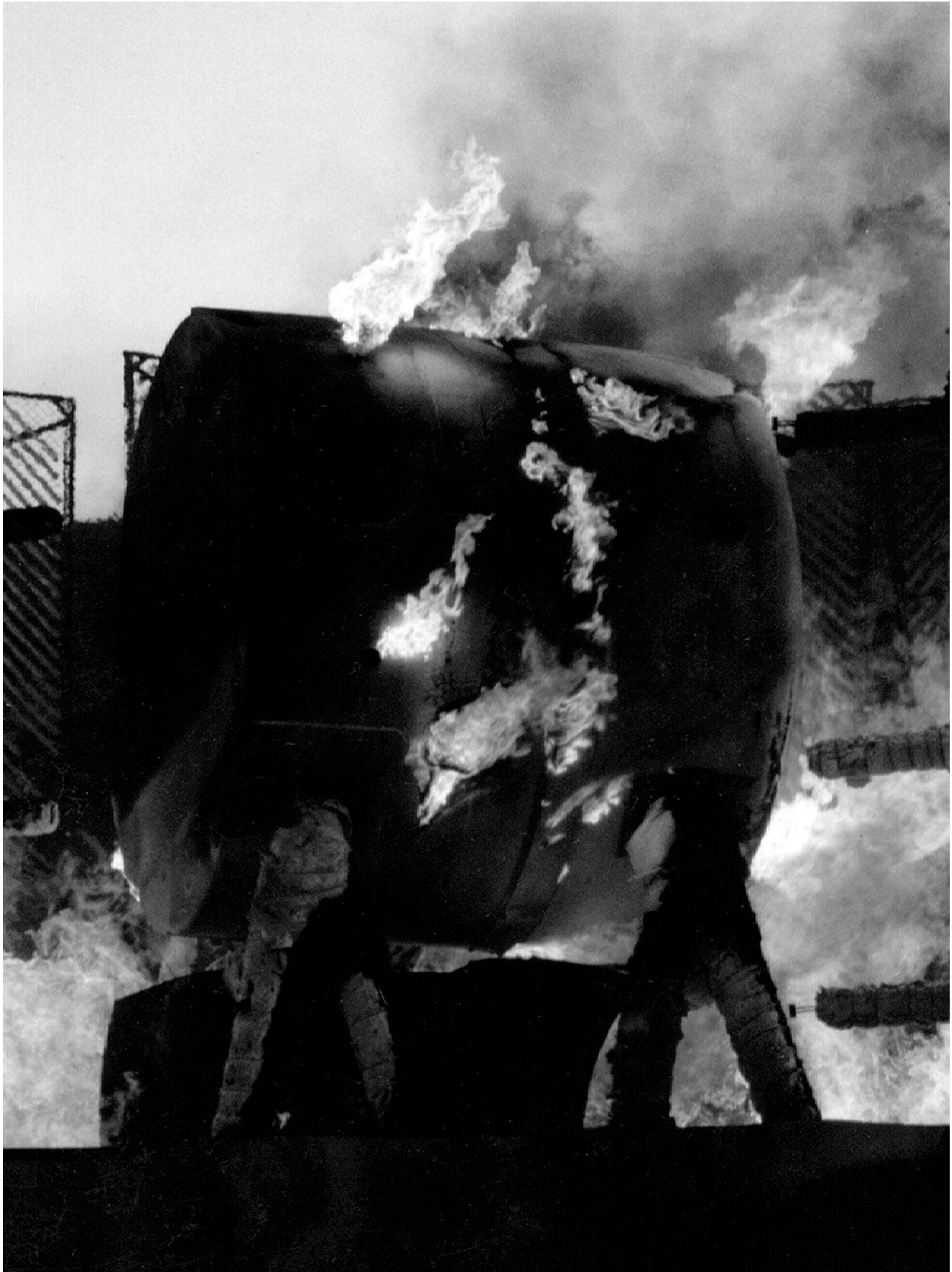
Figure 2.10.3-76 – CTU Fire Test 7; Side 2 View ~33 Minutes after Start (End of Fire)
