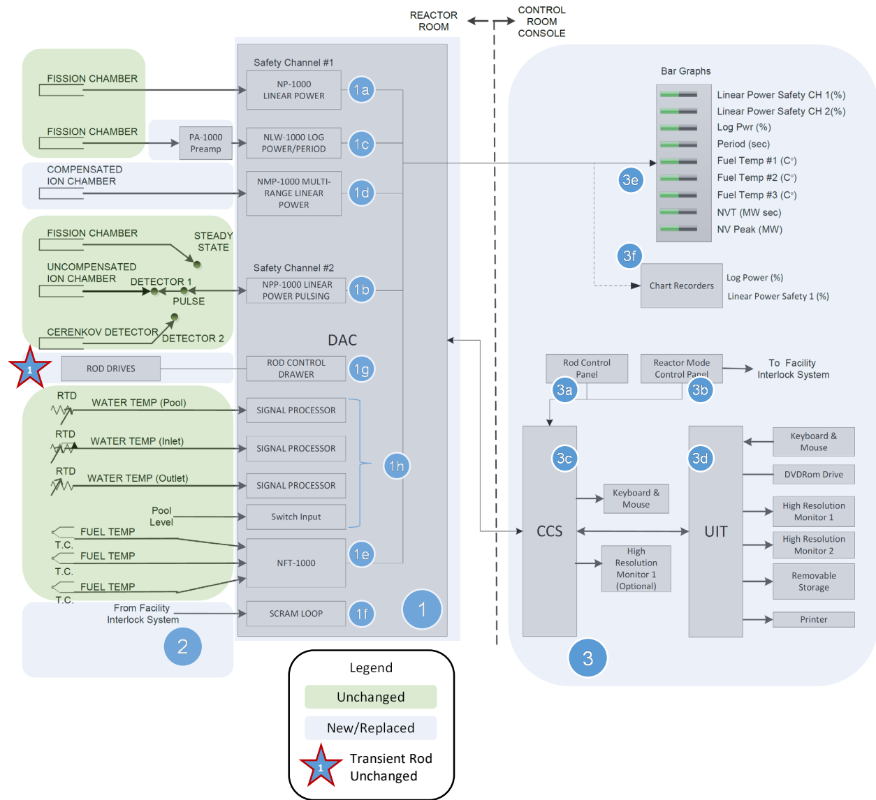
Figure 1 – Diagram of Major Components for the AFRRR Instrumentation and Control System
