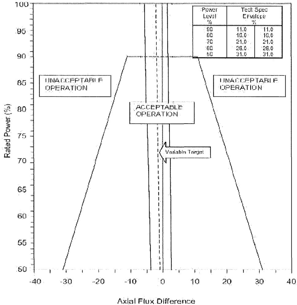
FIGURE 6B FLUX DIFFERENCE OPERATING ENVELOPE (AFD Band of +/- 3%)
