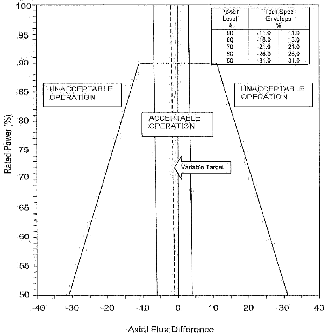
FIGURE 6A FLUX DIFFERENCE OPERATING ENVELOPE (AFD Band of +/- 5%)
