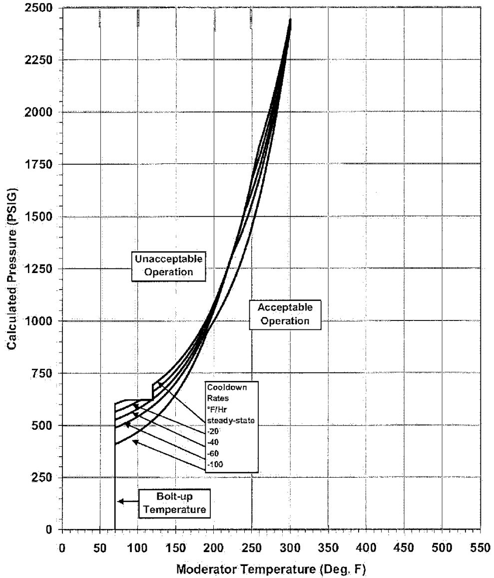
FIGURE 3.4-3 Turkey Point Units 3 & 4 Reactor Coolant System Cooldown Limitations (Cooldown Rates of 0, 20, 40, 60 and 100 °F/hr) Applicable for 48 EFPY (Without Margins for Instrumentation Errors)
